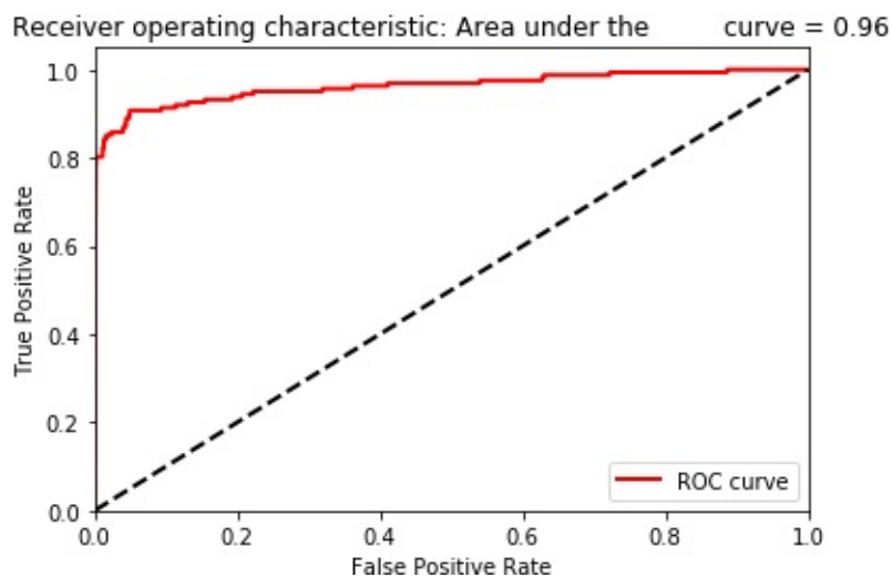
Figure 8-8. Evaluation metrics of sparse overcomplete autoencoder with single hidden layer, dropout, and linear activation function
