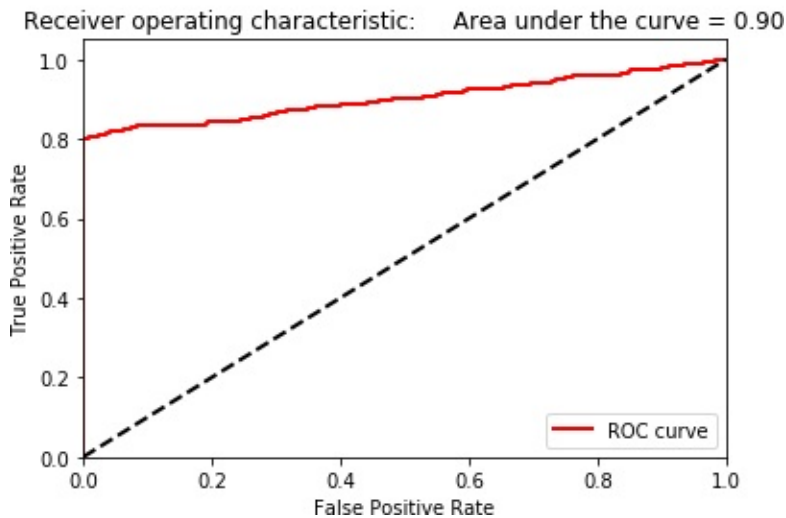
Figure 4-4. Results using normal PCA and 27 principal components
