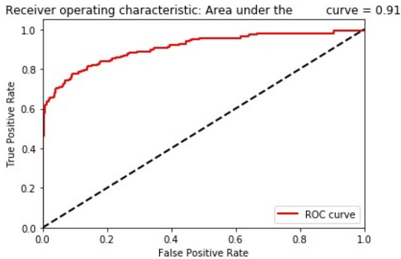
Figure 8-11. Evaluation metrics of denoising overcomplete autoencoder with dropout and ReLU activation function
