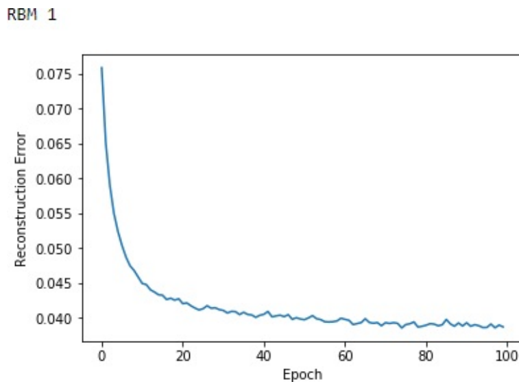
Figure 11-1. Reconstruction errors of first RBM
