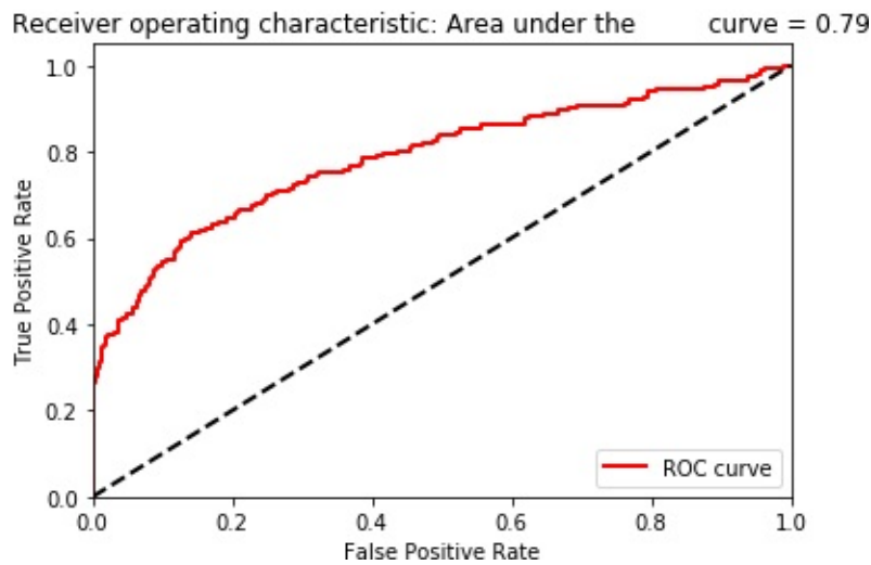
Figure 8-10. Evaluation metrics of denoising overcomplete autoencoder with dropout and linear activation function
