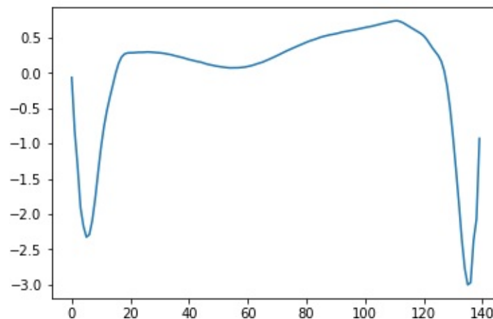
Figure 13-6. ECG5000 class 2.0
