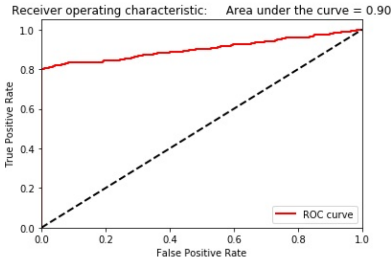
Figure 4-16. Results using ICA and 27 components
