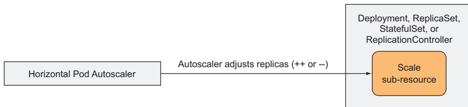
Figure 15.3 The Horizontal Pod Autoscaler modifies only on the Scale sub-resource.
