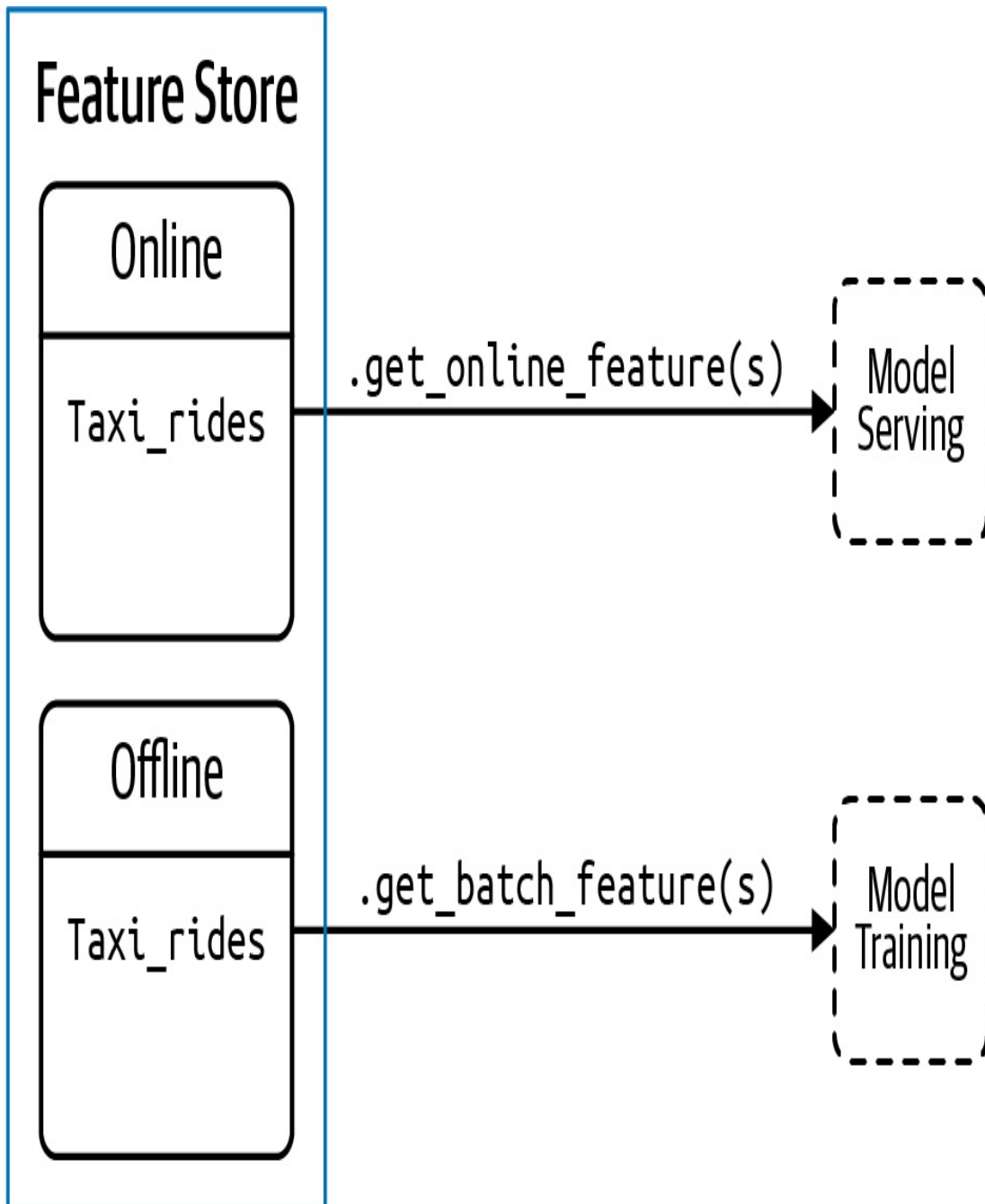
Figure 6-15. Feature data can be retrieved either offline, using historical features for model training, or online, for serving.
