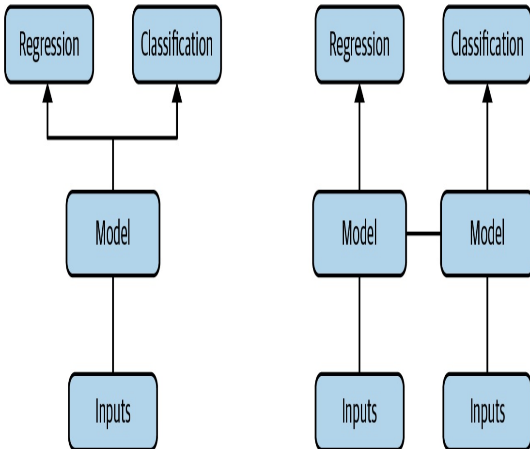
Figure 3-6. Two common implementations of multitask learning are through hard parameter sharing and soft parameter sharing.
