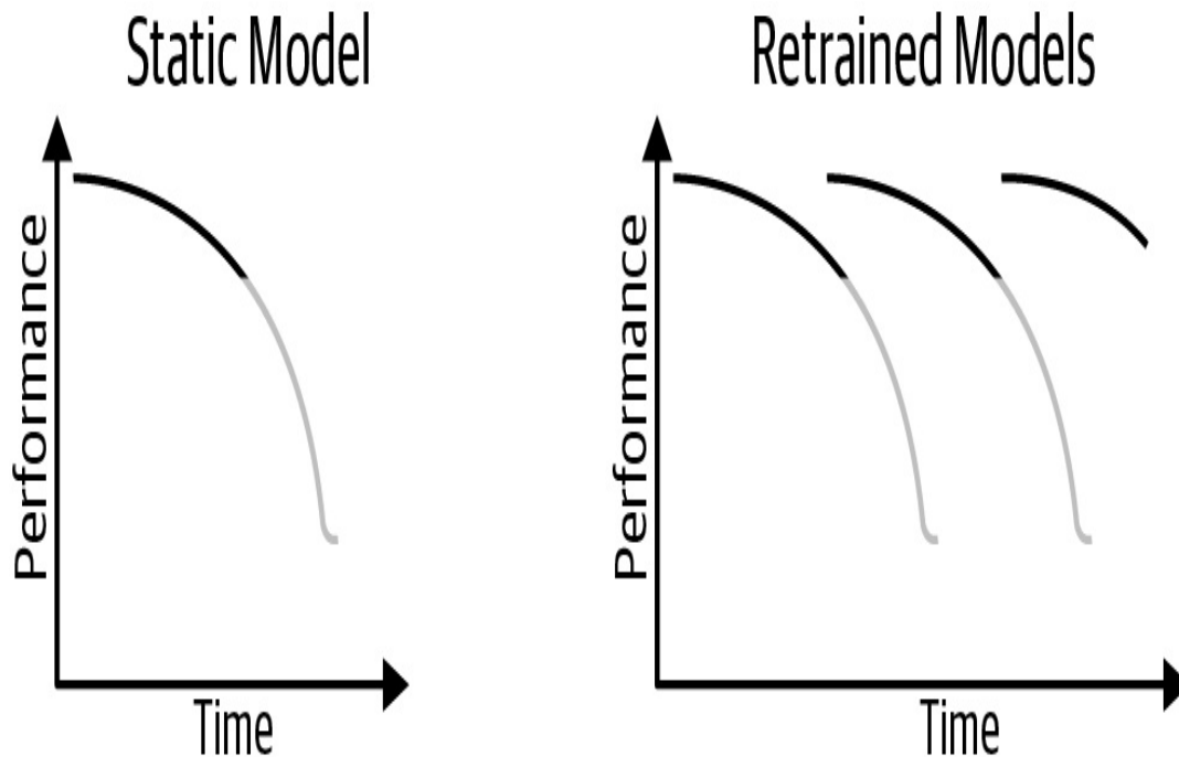
Figure 8-3. Model staleness can occur for many reasons. Retraining models periodically can help to improve their performance over time.
