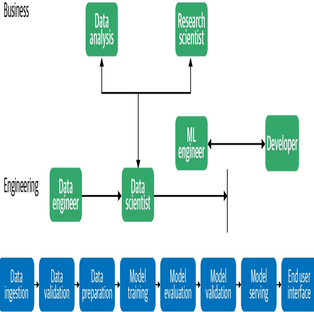
Figure 1-2. There are many different job roles related to data and machine learning, and these roles collaborate on the ML workflow, from data ingestion to model serving and the end user interface. For example, the data engineer works on data ingestion and data validation and collaborates closely with data scientists.
