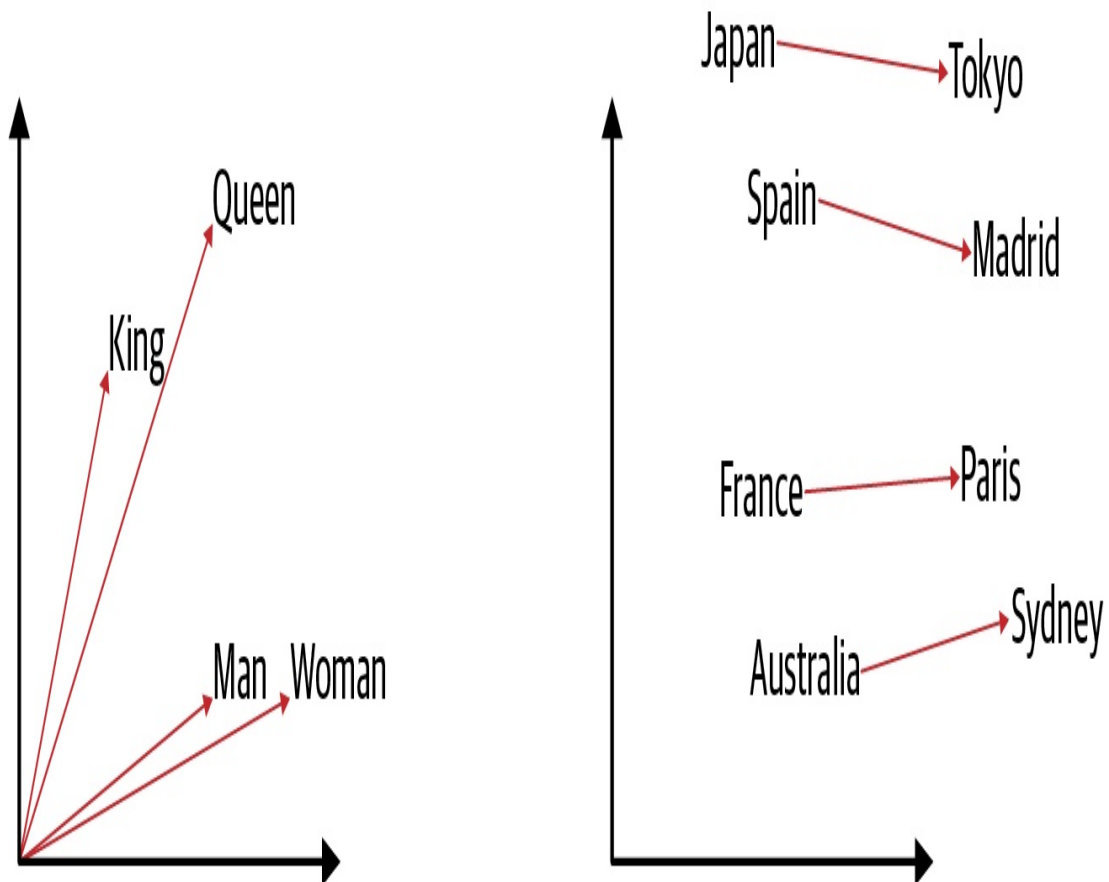
Figure 2-12. Word embeddings capture semantic relationships.
