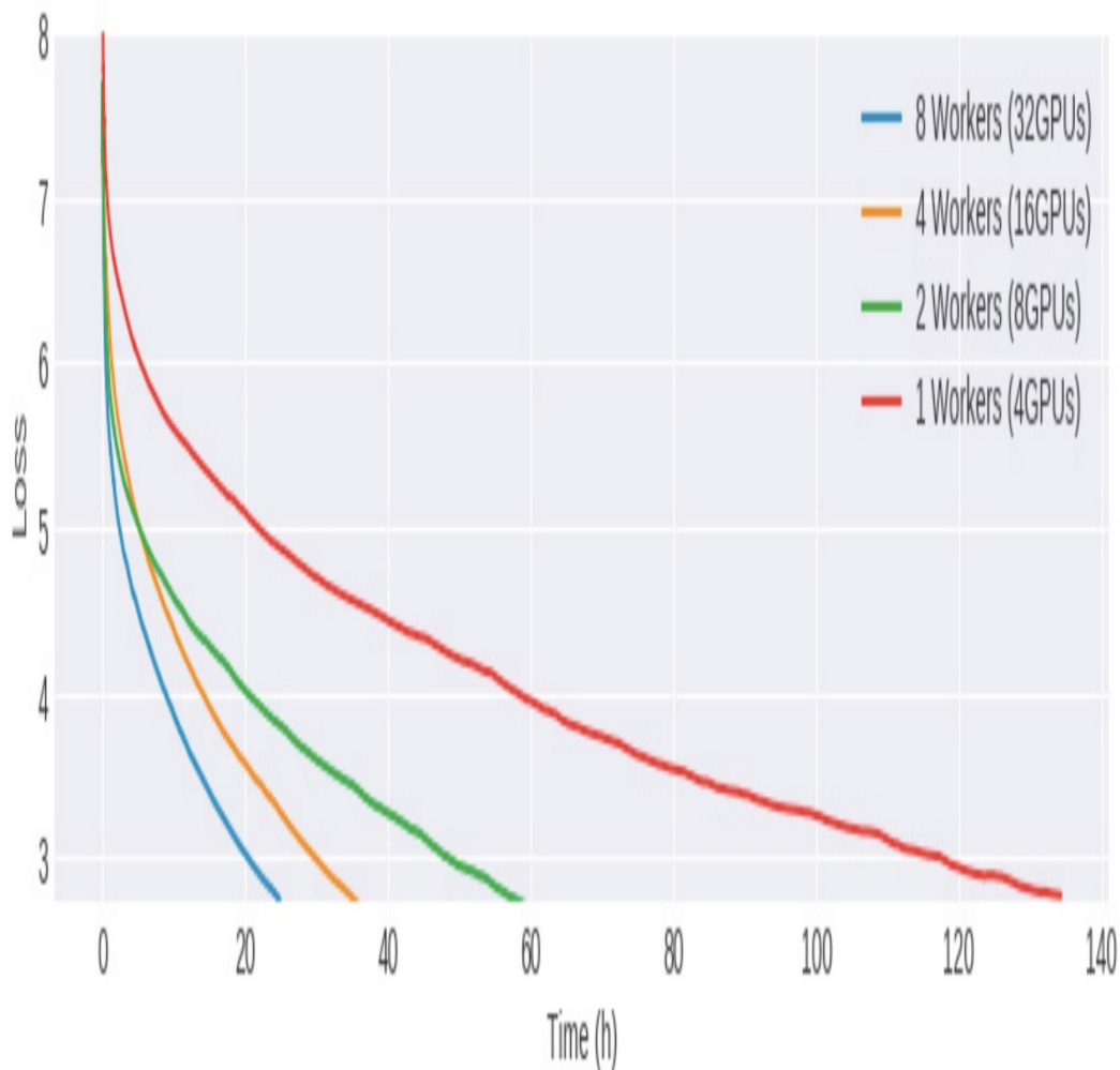
Figure 4-18. As the number of GPUs increases, the time to convergence during training decreases.
