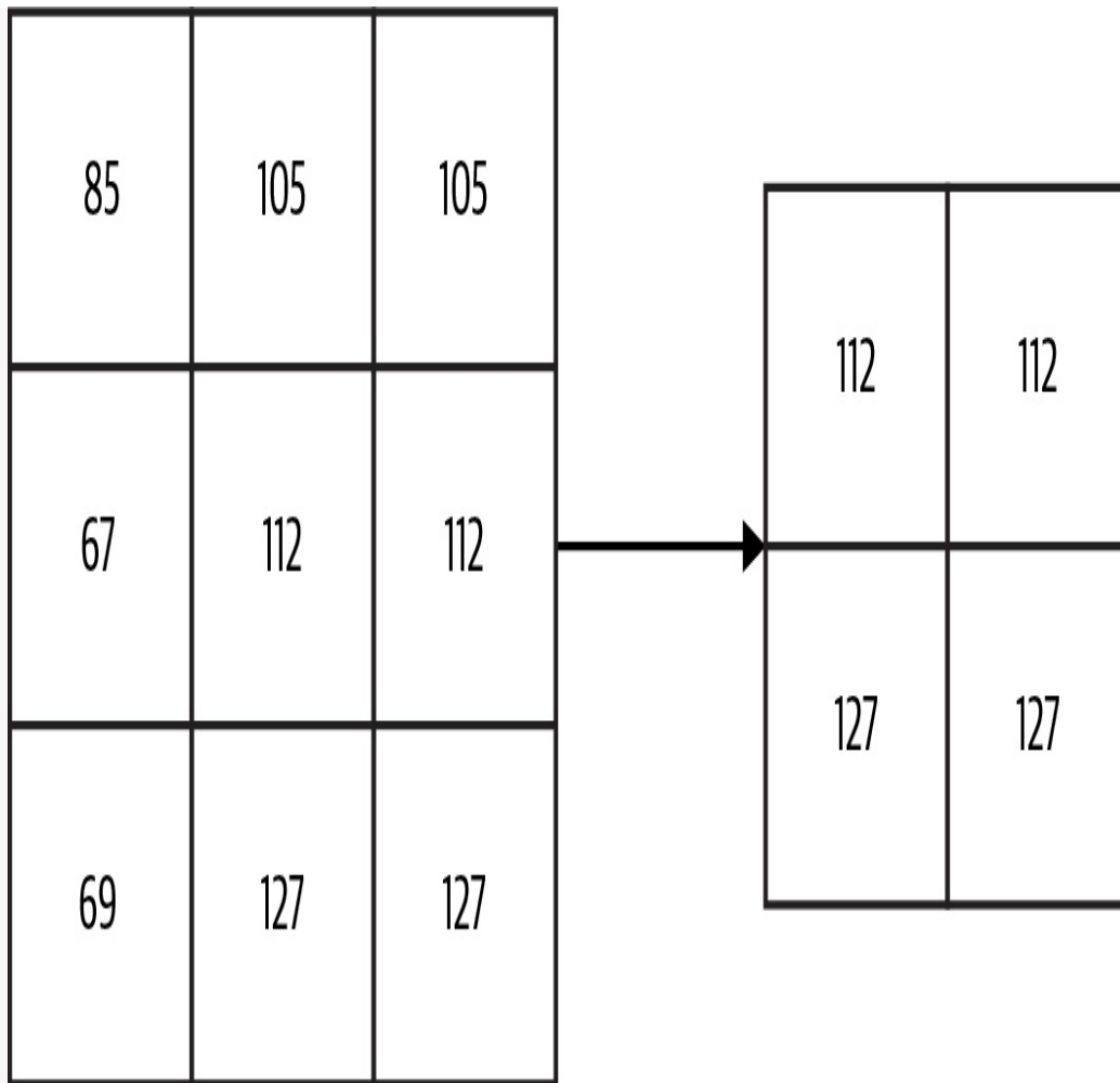
Figure 2-24. Transforming the 3×3 grid into 2×2 with sliding windows and max pooling.
