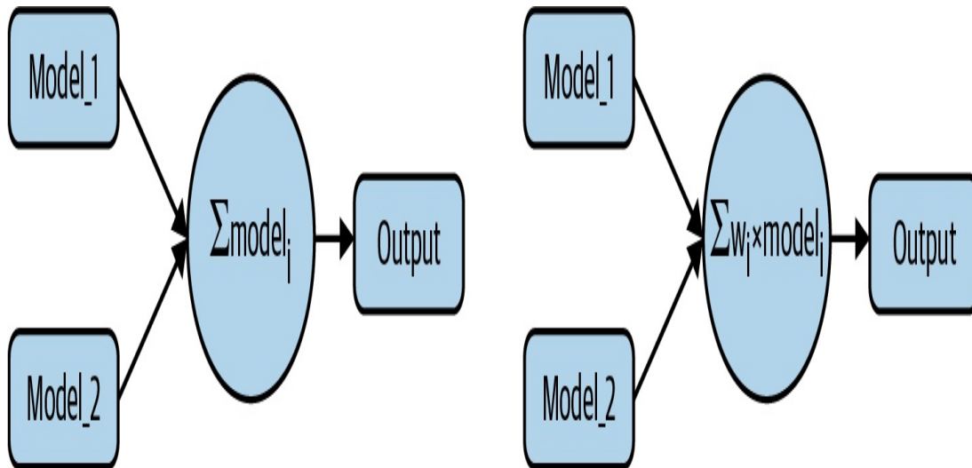
Figure 3-14. The simplest form of model averaging averages the outputs of two or more different machine learning models. Alternatively, the average could be replaced with a weighted average where the weight might be based on the relative accuracy of the models.
