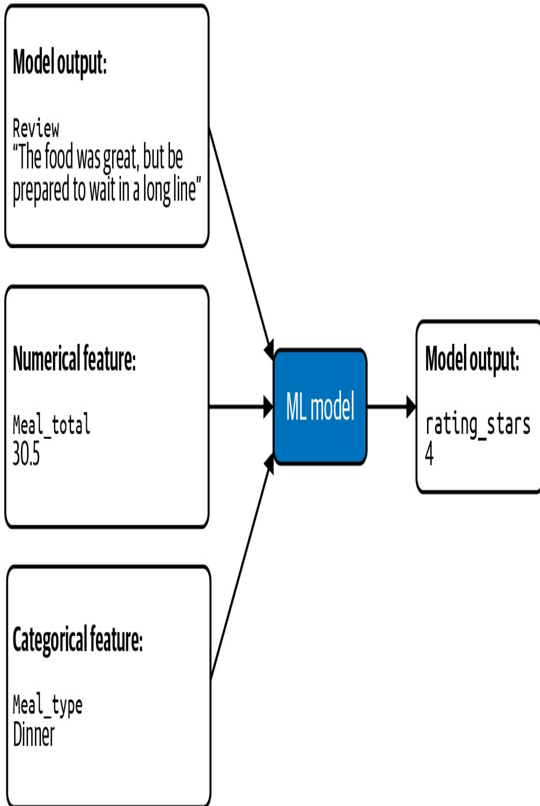
Figure 2-20. Model combining free-form text input with tabular data to predict the rating of a restaurant review.
