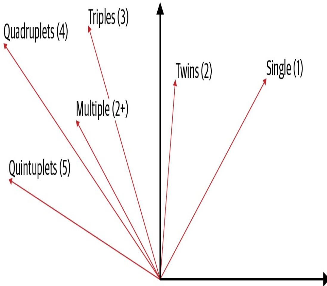
Figure 2-9. By forcing our categorical variable into a lower-dimensional embedding space, we can also learn relationships between the different categories.
