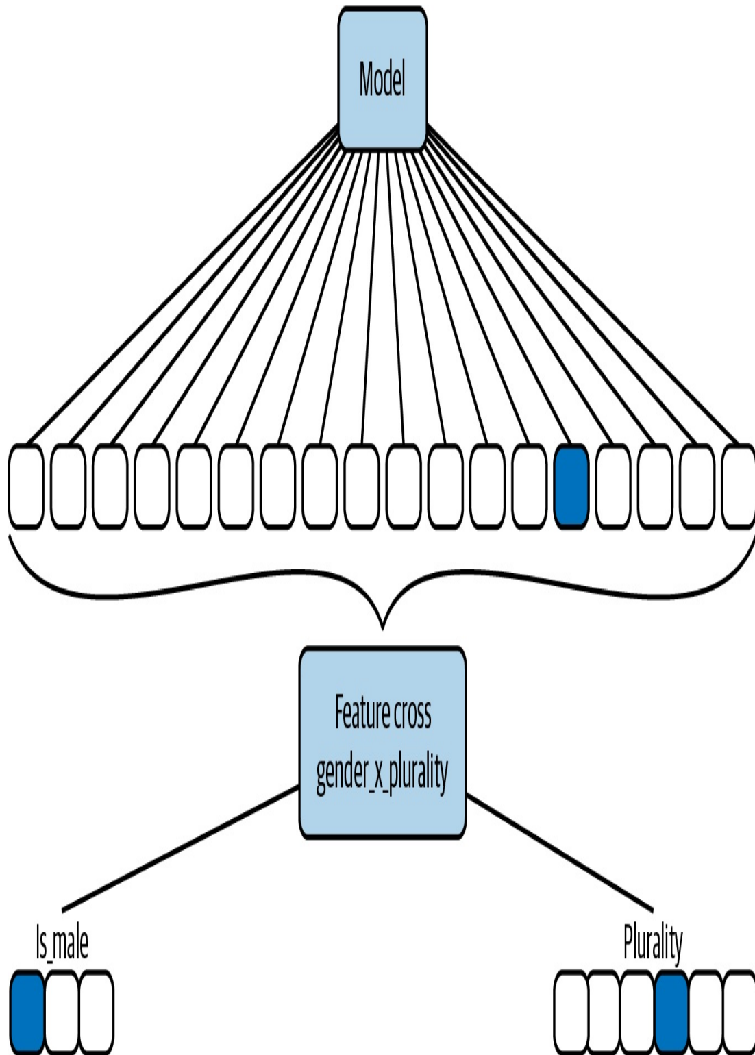
Figure 2-16. A feature cross between is_male and plurality creates an additional 18 binary features in our ML model.
