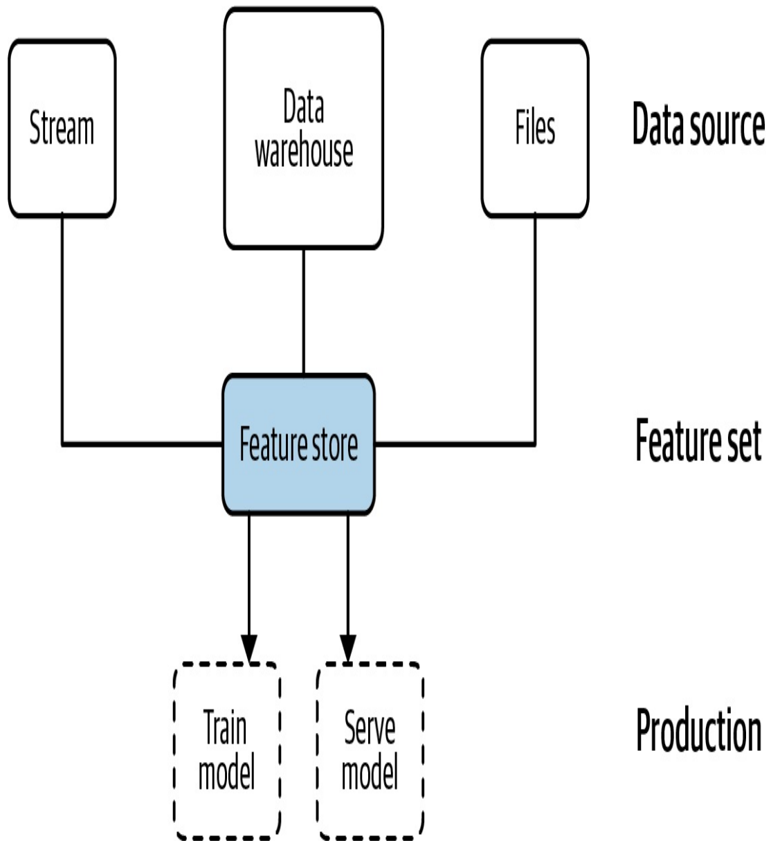
Figure 6-16. A feature store ensures the feature engineering pipelines are consistent between model training and serving. See also https://docs.feast.dev/ .
