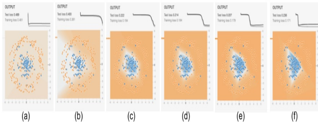
Figure 4-8. What the model learns as training progresses. The graphs at the top are the training loss and validation error, while the images show how the model at that stage would predict the color of a point at each coordinate in the grid.
