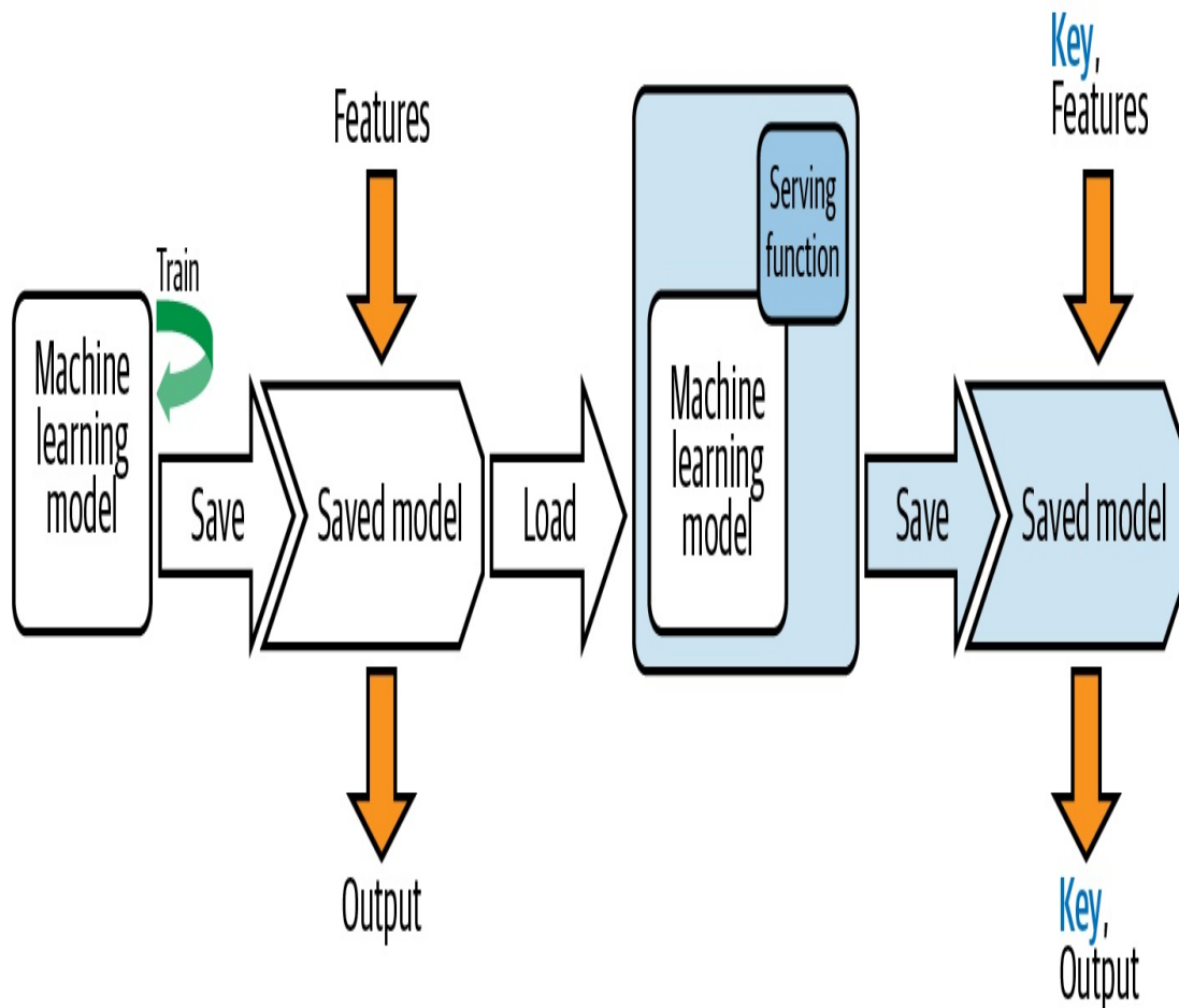
Figure 5-14. Load a SavedModel, attach a nondefault serving function, and save it.
