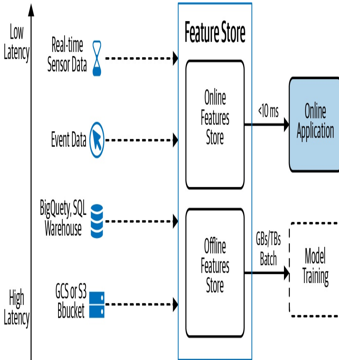
Figure 6-18. The Feature Store design pattern can handle both the requirements of data being highly scalable for large batches during training and extremely low latency for serving online applications.
