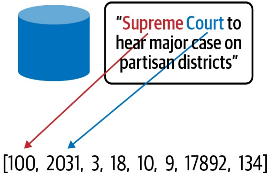
Figure 2-7. Using the tokenizer, each title is mapped to a sequence of integer index values.
