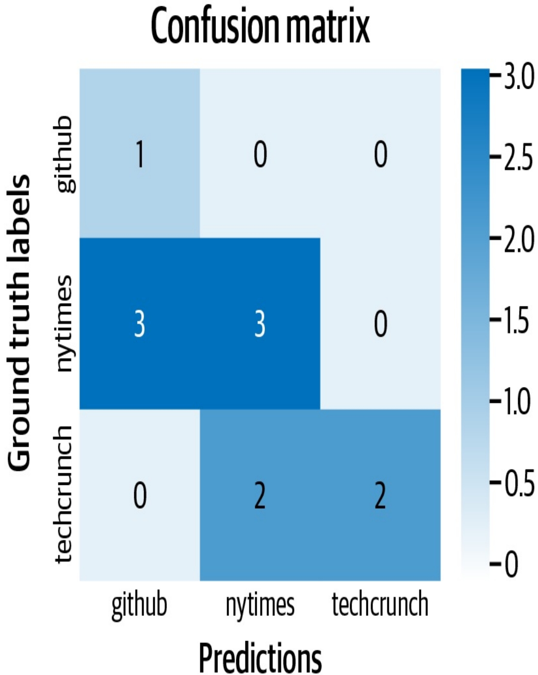
Figure 5-3. A confusion matrix shows all pairs of ground truth labels and predictions so you can explore your model performance within different classes.
