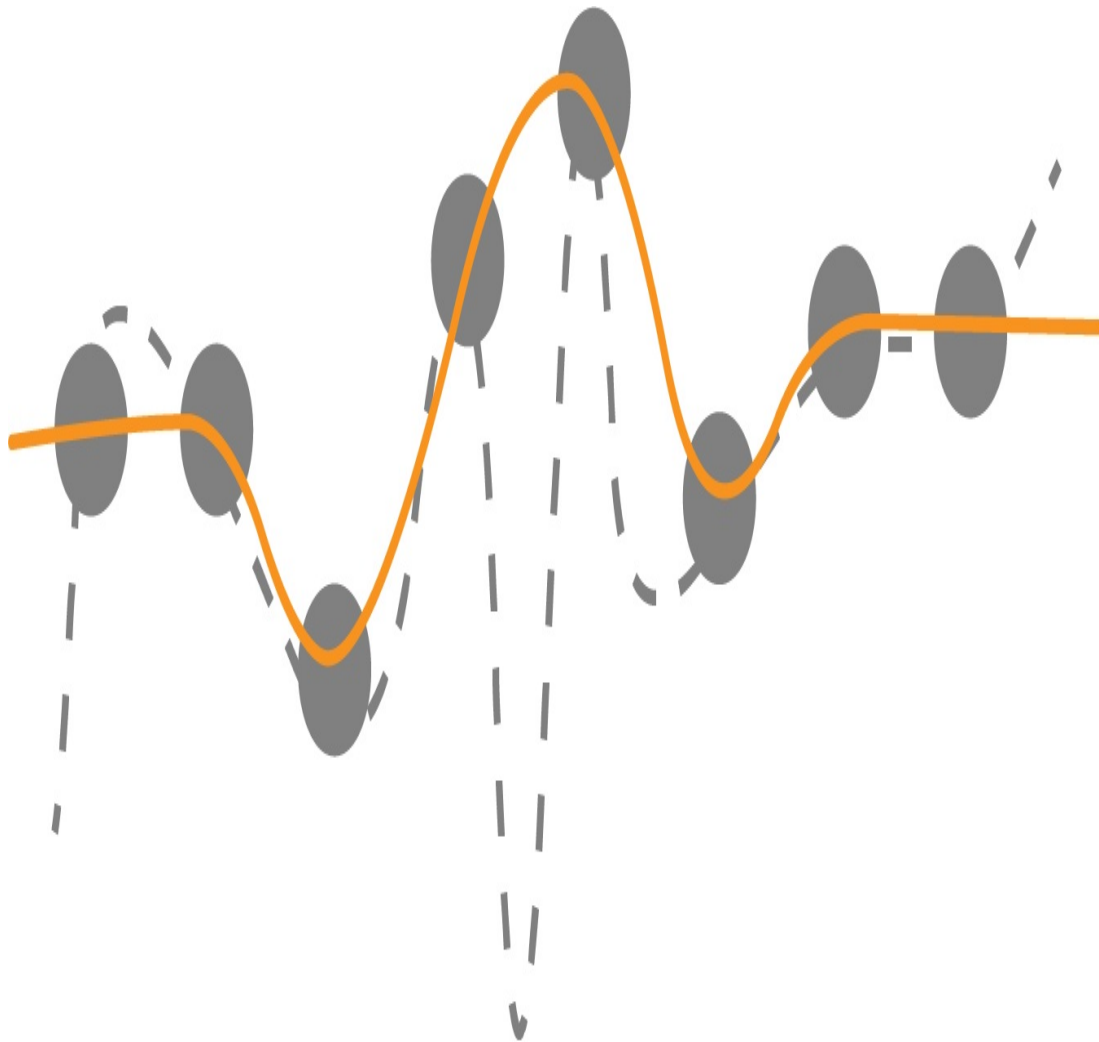
Figure 4-4. Overfitting is not a concern if all possible input points are trained for because predictions are the same with both curves.
