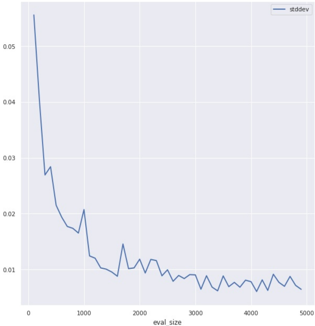
Figure 6-3. Determine the number of evaluation examples needed by evaluating the production model on subsets of varying sizes and tracking the variability of the evaluation metric by the size of the subset. Here, the standard deviation starts to plateau at around 2,000 examples.
