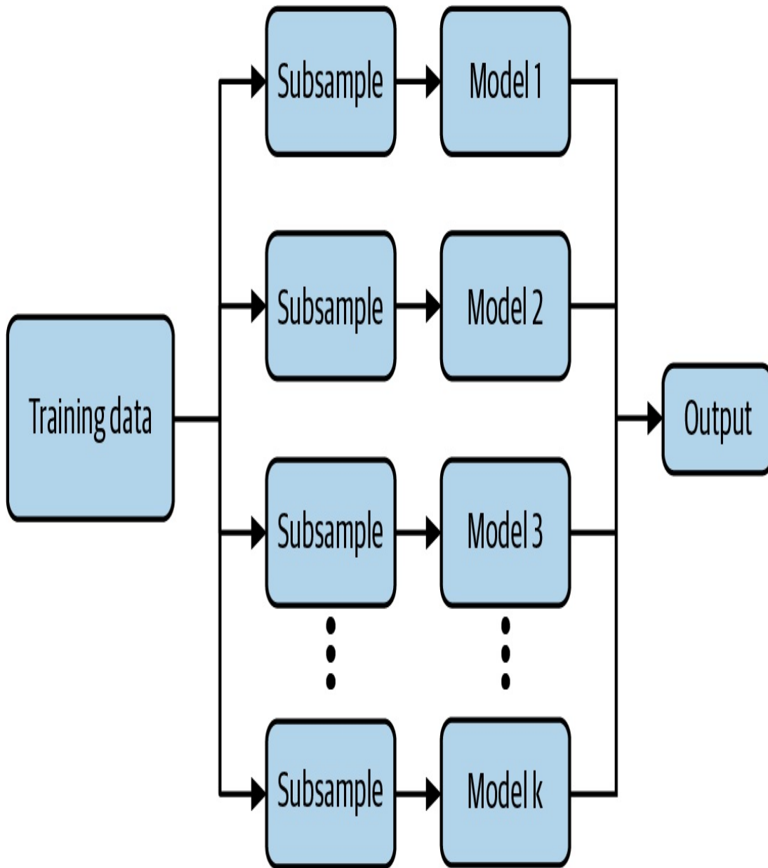
Figure 3-11. Bagging is good for decreasing variance in machine learning model output.
