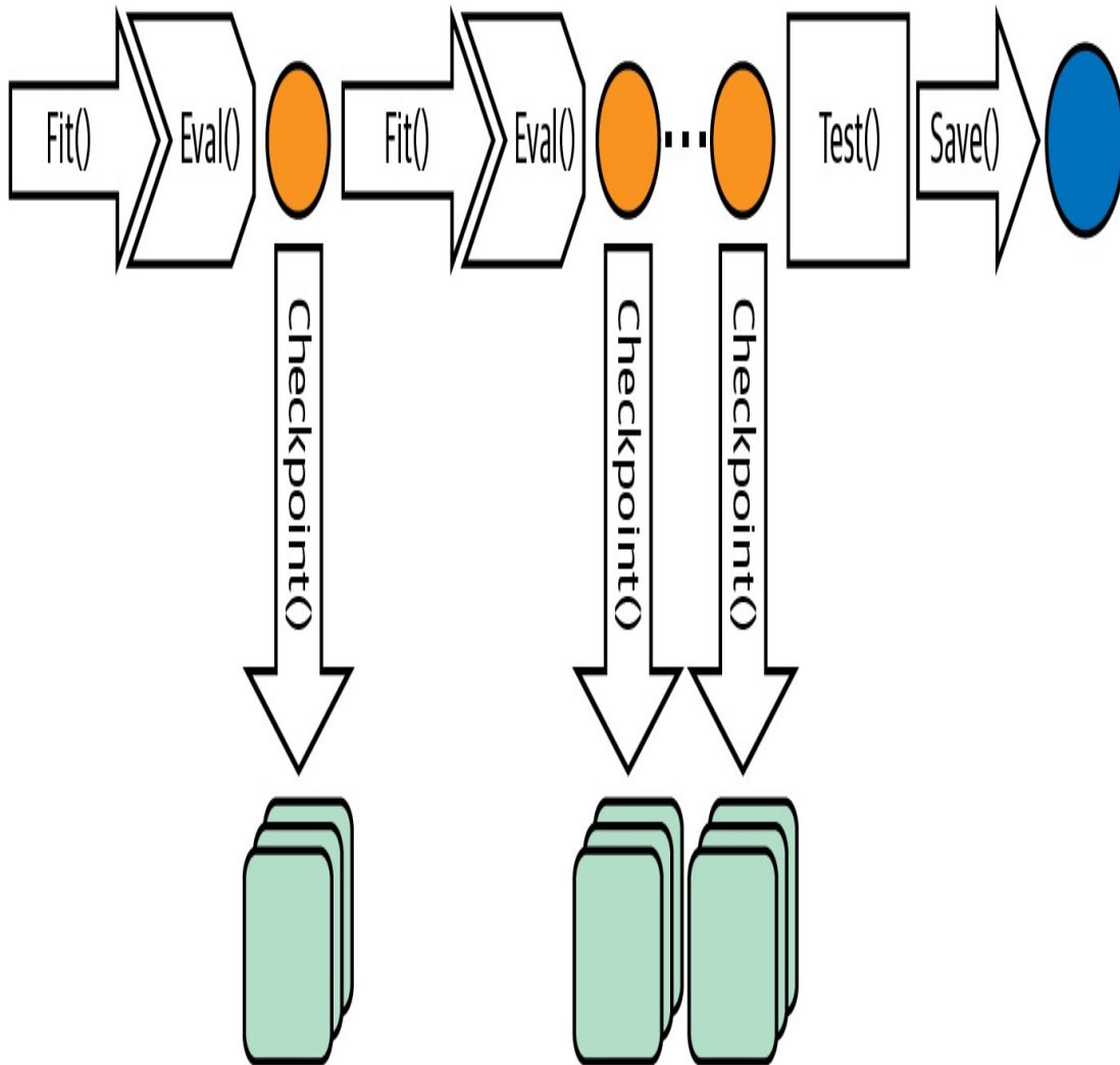
Figure 4-6. Checkpointing saves the full model state at the end of every epoch.
