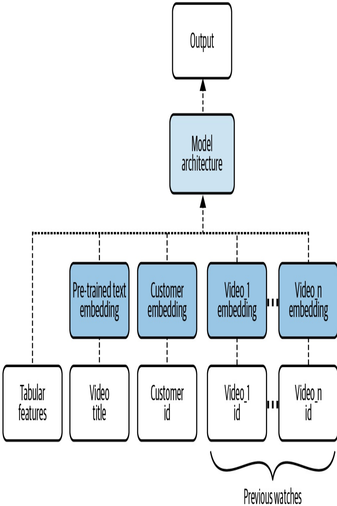
Figure 2-13. A pre-trained text embedding can be added to a model to process text features.
