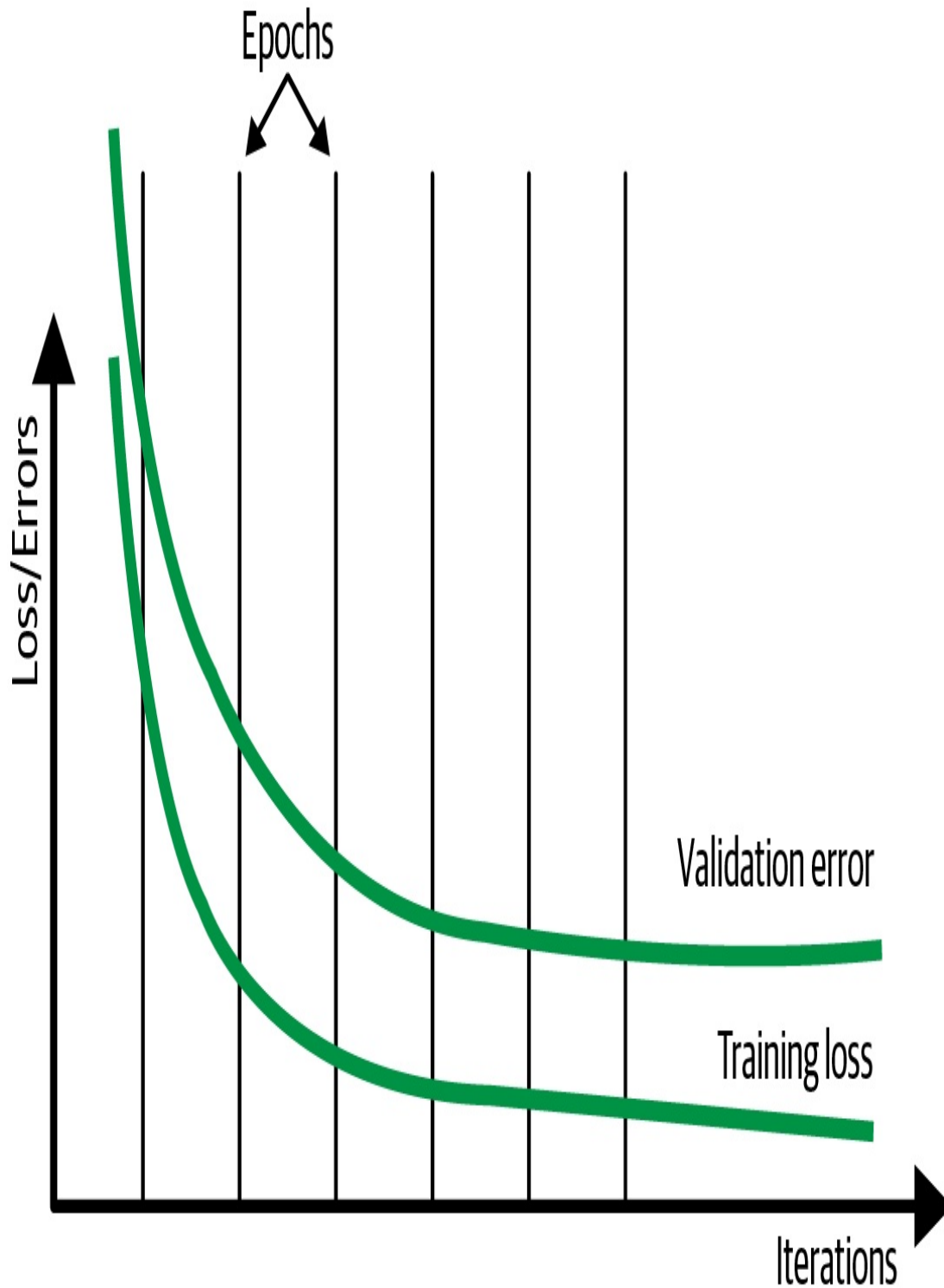
Figure 4-10. In the ideal situation, validation error does not increase. Instead, both the training loss and validation error plateau.
