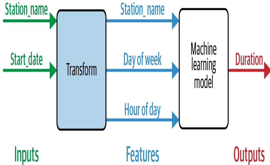
Figure 6-1. The model has three features computed from two inputs.
