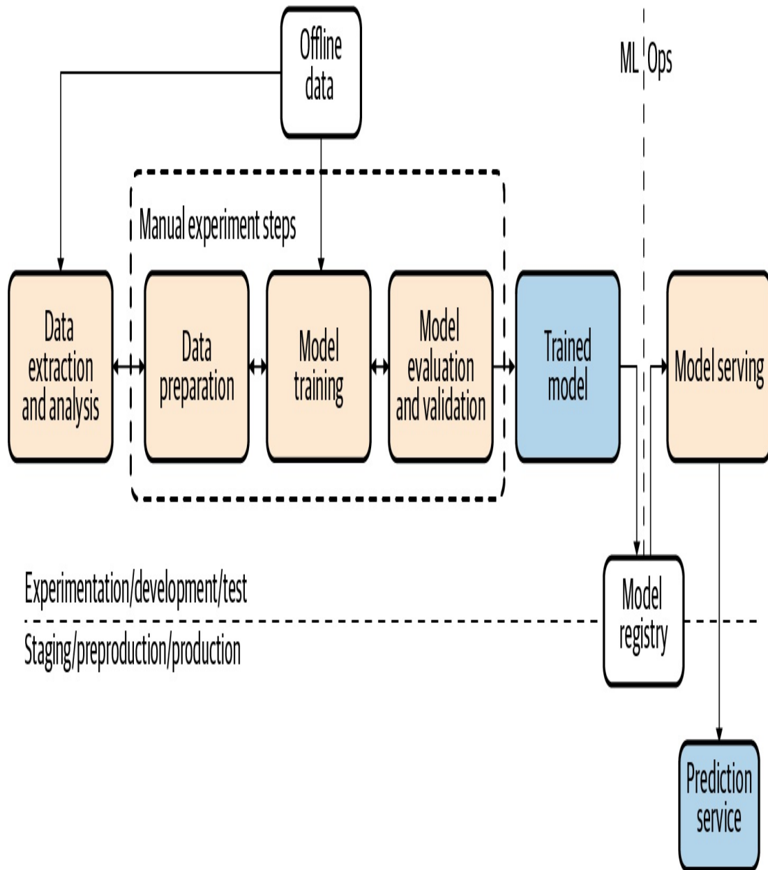
Figure 8-4. Manual development of AI models. Figure adapted from Google Cloud documentation .
