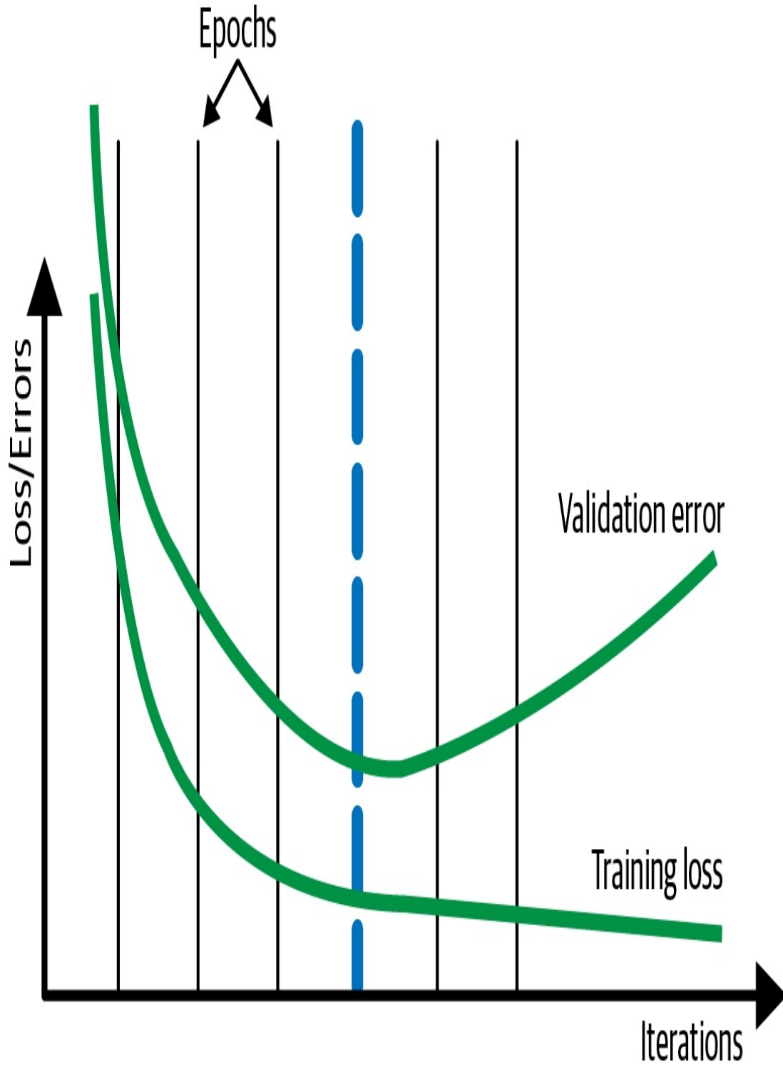
Figure 4-9. Typically, the training loss continues to drop the longer you train, but once overfitting starts, the validation error on a withheld dataset starts to go up.
