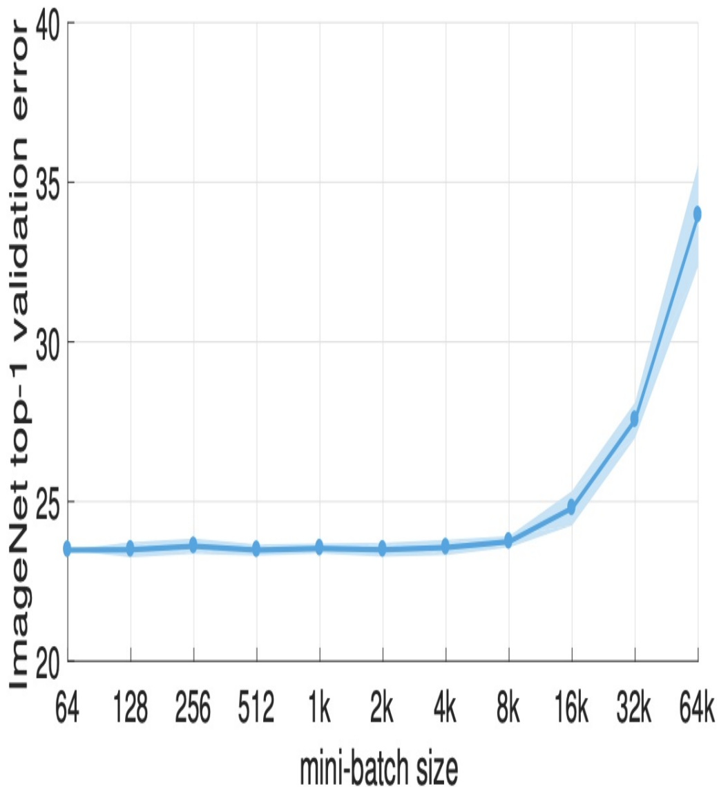
Figure 4-20. Large batch sizes have been shown to adversely affect the quality of the final trained model.
