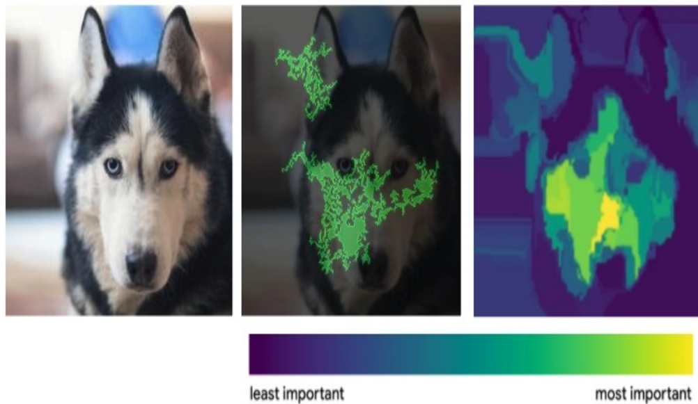
Figure 7-5. The feature attributions returned from Explainable AI for an ImageNet model deployed to AI Platform. On the left is the original image. The IG attributions are shown in the middle, and the XRAI attributions are shown on the right. The key below shows what the regions in XRAI correspond to—lighter regions are the most important, and darker areas represent the least important regions.
