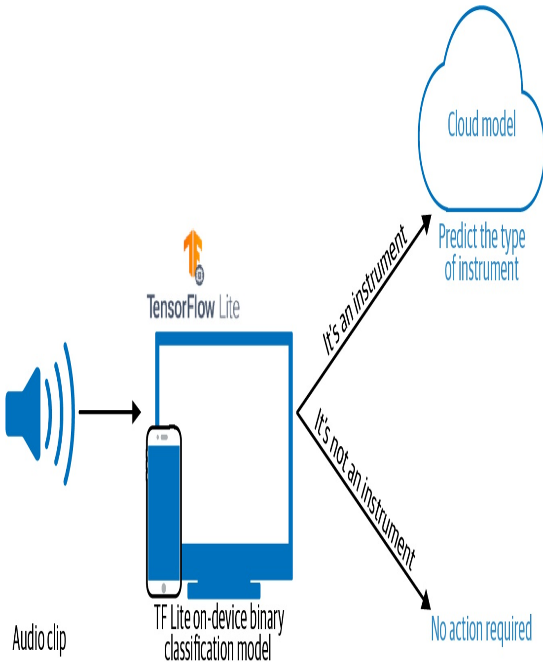
Figure 5-10. Using the Two-Phase Predictions pattern to identify instrument sounds.
