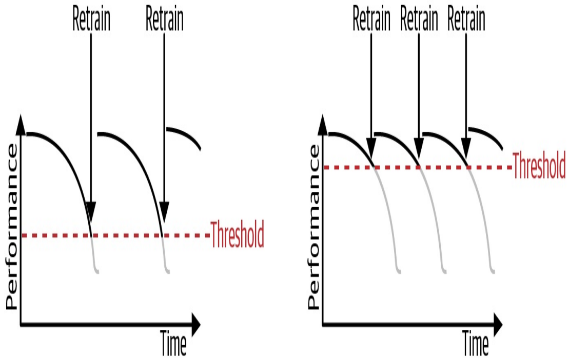
Figure 5-5. Setting a higher threshold for model performance ensures a higher-quality model in production but will require more frequent retraining jobs, which can be costly.
