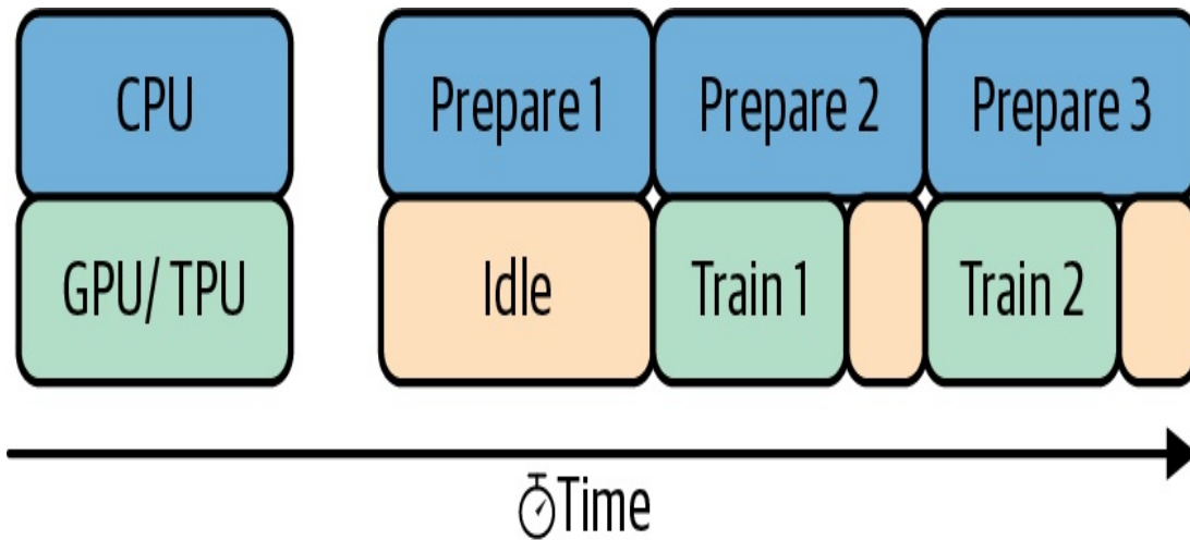
Figure 4-22. Prefetching overlaps preprocessing and model execution, so that while the model is executing one training step, the input pipeline is reading and preparing data for the next.
