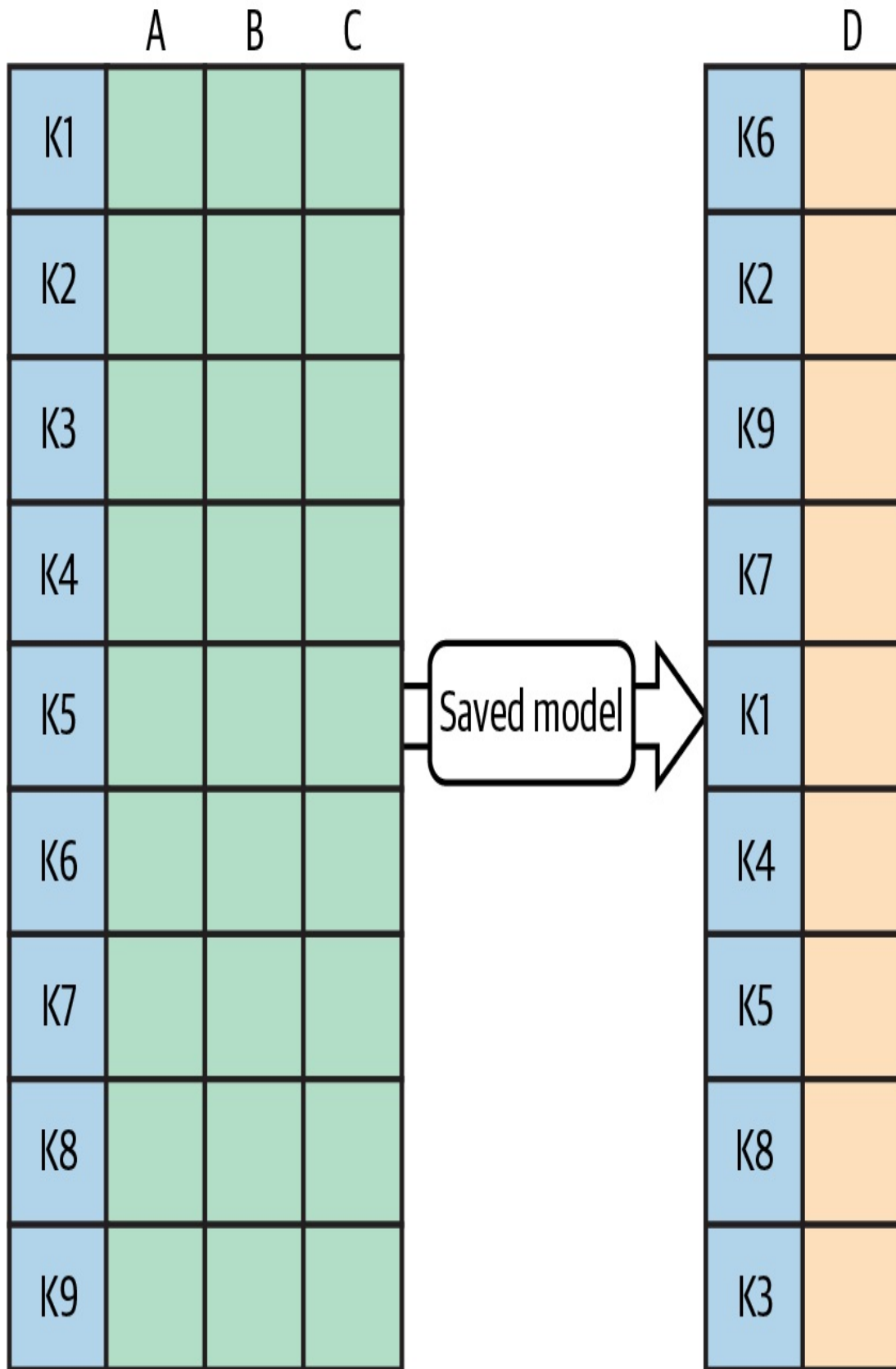
Figure 5-13. The client supplies a unique key with each input instance. The serving system attaches
