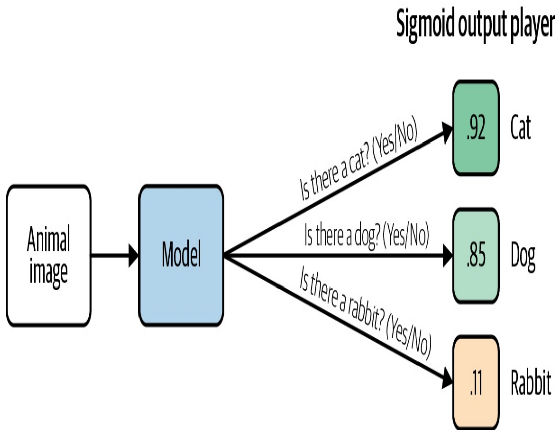
Figure 3-9. Understanding the Multilabel pattern by breaking down the problem into smaller binary classification tasks.
