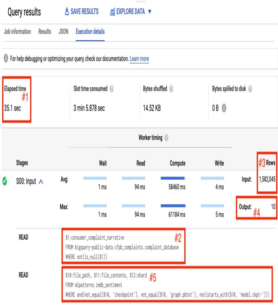
Figure 5-1. The first two steps of a query to find the five most “positive” complaints in the Consumer Financial Protection Bureau dataset of consumer complaints.
