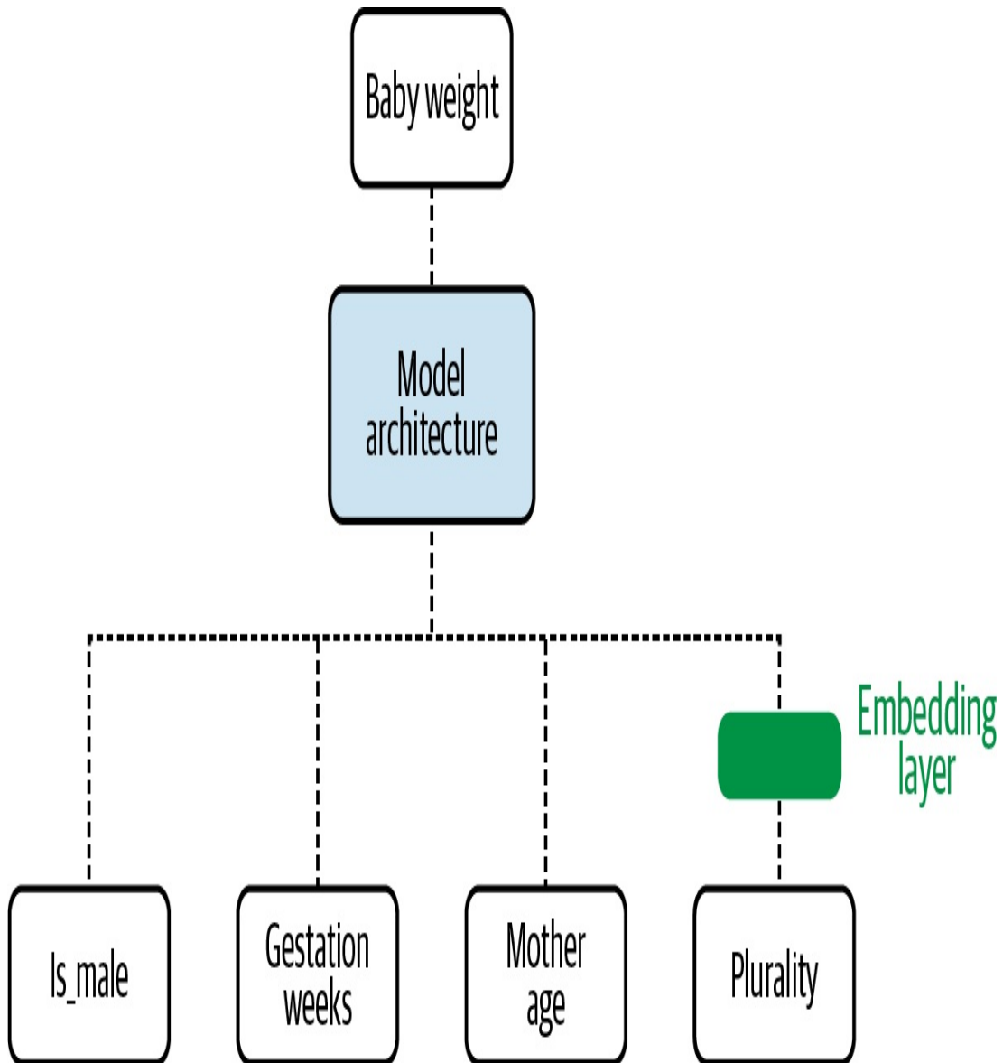
Figure 2-5. The weights of an embedding layer are learned as parameters during training.
