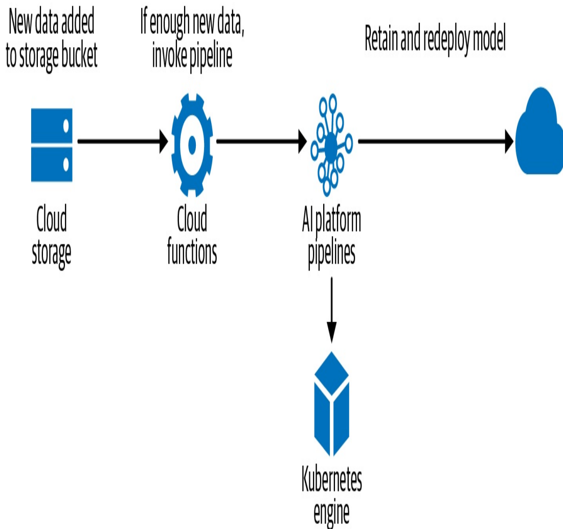
Figure 6-9. A CI/CD workflow using Cloud Functions to invoke a pipeline when enough new data is added to a storage location.
