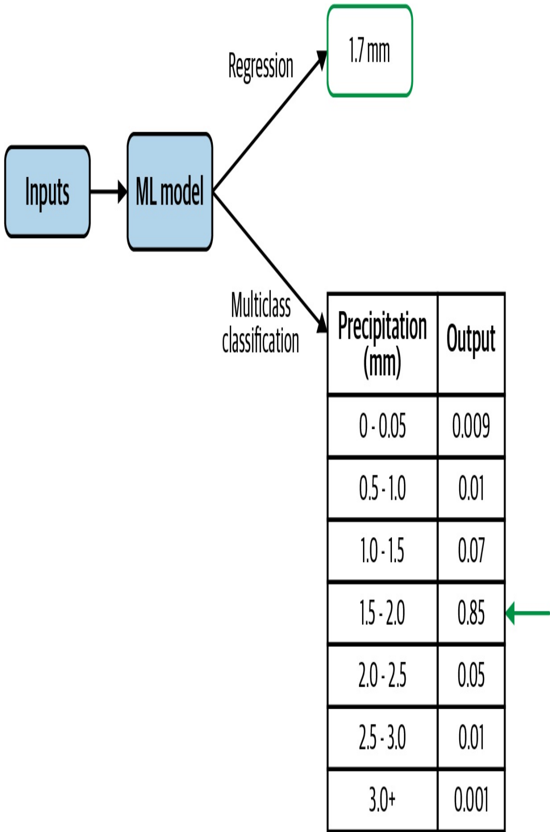
Figure 3-1. Instead of predicting precipitation as a regression output, we can instead model
