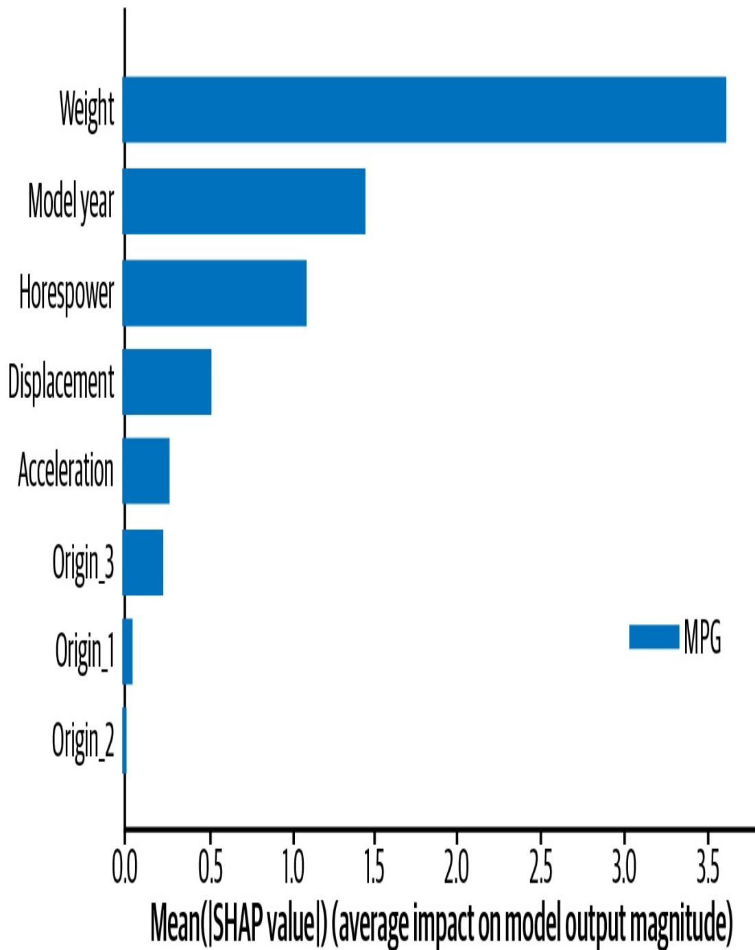
Figure 7-4. An example of global-level feature attributions for the fuel efficiency model, calculated on the first 10 examples from the test dataset.
