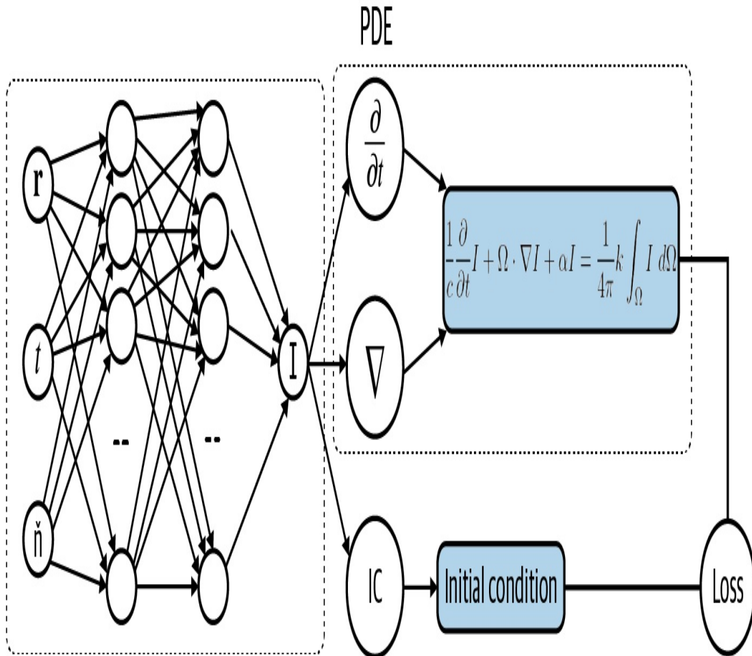
Figure 4-3. Architecture for using a neural network to model the solution of a partial differential equation to solve for I(r,t,n) .
