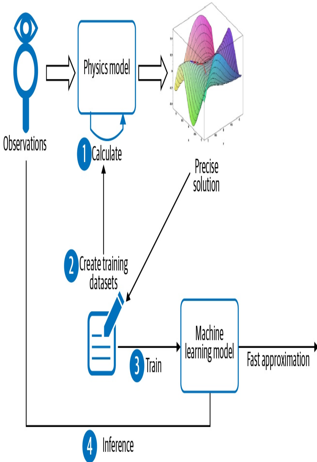
Figure 4-2. One situation when it is acceptable to overfit is when the entire domain space of observations can be tabulated and a physical model capable of computing the precise solution is available.
