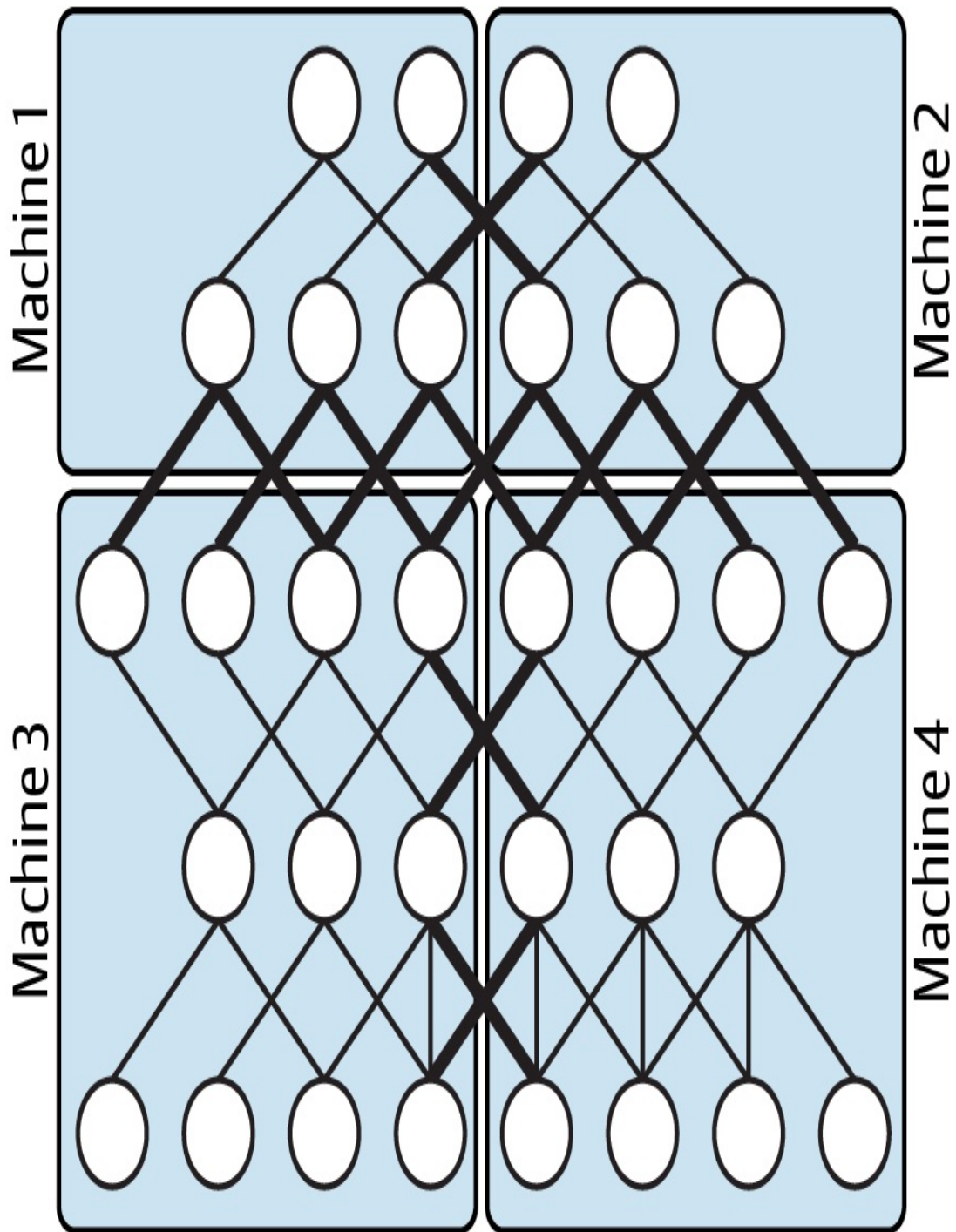
Figure 4-19. Model parallelism partitions the model over multiple devices.
