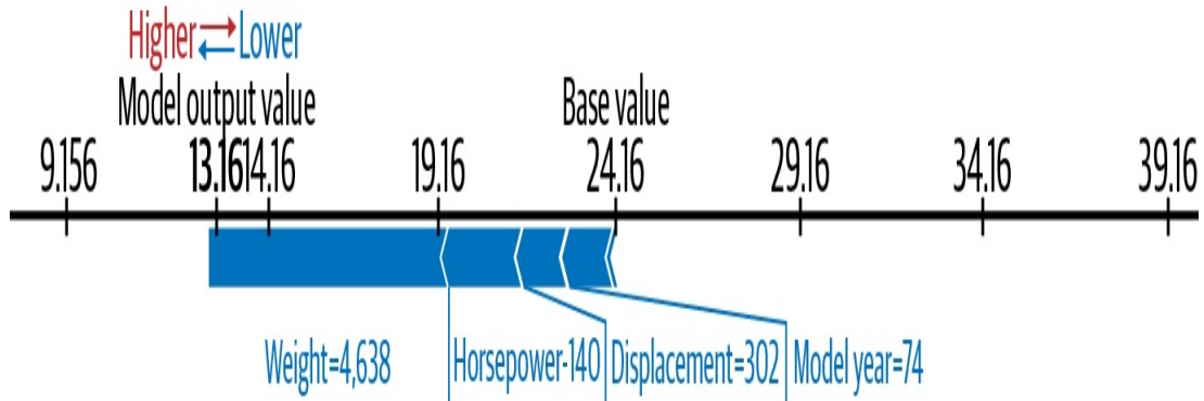
Figure 7-3. The feature attribution values for one example from our fuel efficiency prediction model. In this case, the car's weight is the most significant indicator of MPG with a feature attribution value of roughly 6. Had our model's prediction been above the baseline of 24.16, we would instead see mostly negative attribution values.
