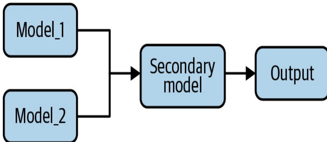
Figure 3-15. Stacking is an ensemble learning technique that combines the outputs of several different ML models as the input to a secondary ML model that makes predictions.
