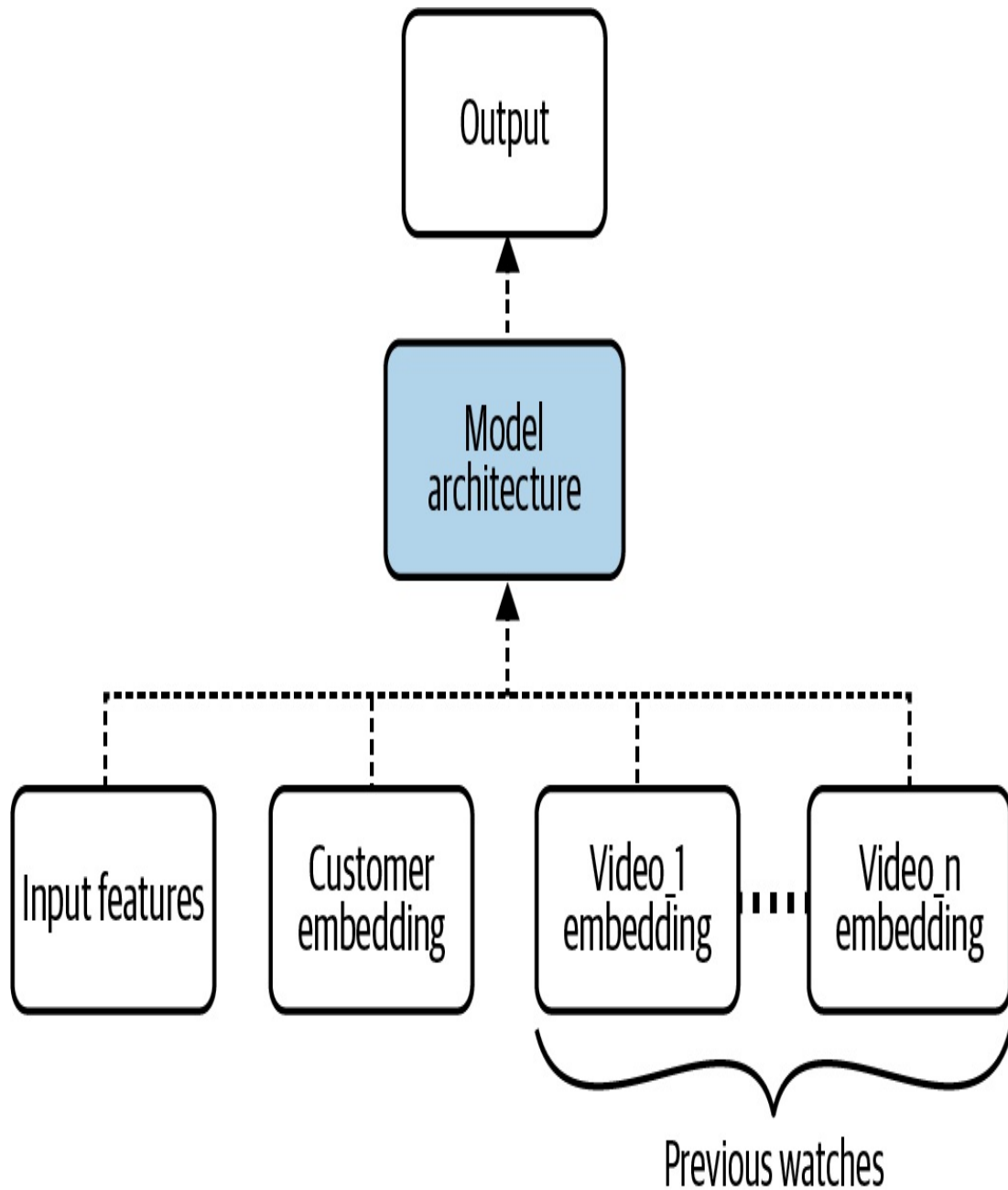
Figure 2-10. By learning a low-dimensional, dense embedding vector for each customer and video, an embedding-based model is able to generalize well with less of a manual feature engineering burden.
