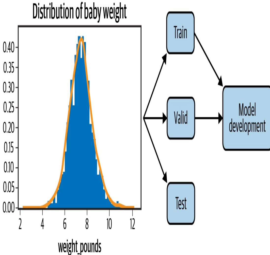
Figure 5-4. When developing a machine learning model, the train, validation, and test data come from the same data distribution. However, once the model is deployed, that distribution can change, severely affecting model performance.
