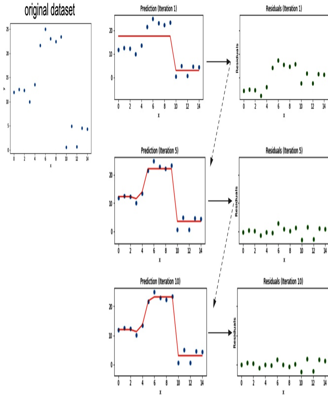
Figure 3-12. Boosting converts weak learners into strong learners by iteratively improving the model prediction.
