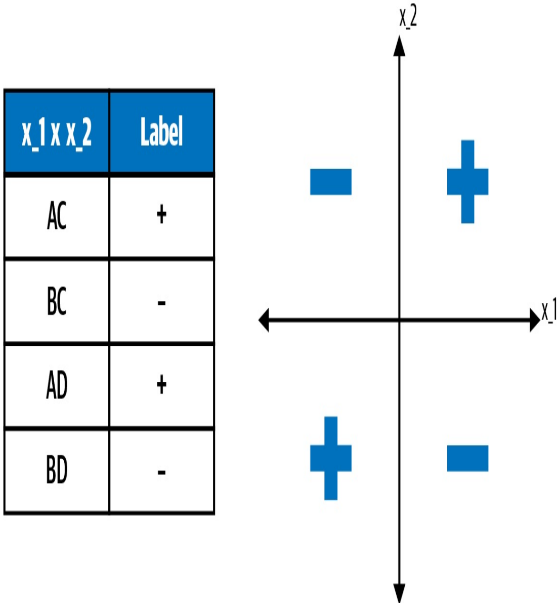
Figure 2-15. The feature cross introduces four new boolean features.
