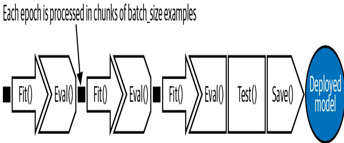
Figure 4-1. A typical training loop consisting of three epochs. Each epoch is processed in chunks of batch_size examples. At the end of the third epoch, the model is evaluated on the testing dataset, and saved for potential deployment as a web service.
