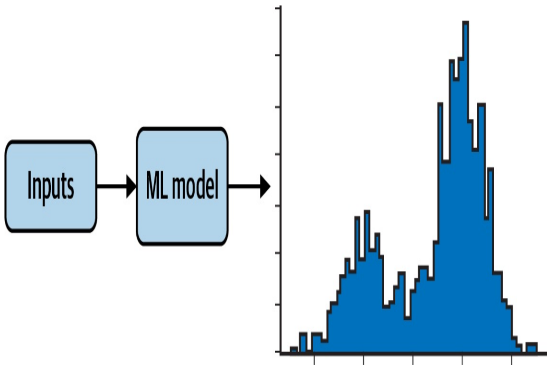
Figure 3-2. Reframing a classification task to model a probability distribution allows the predictions to capture bimodal output. The prediction is not limited to a single value as in a
