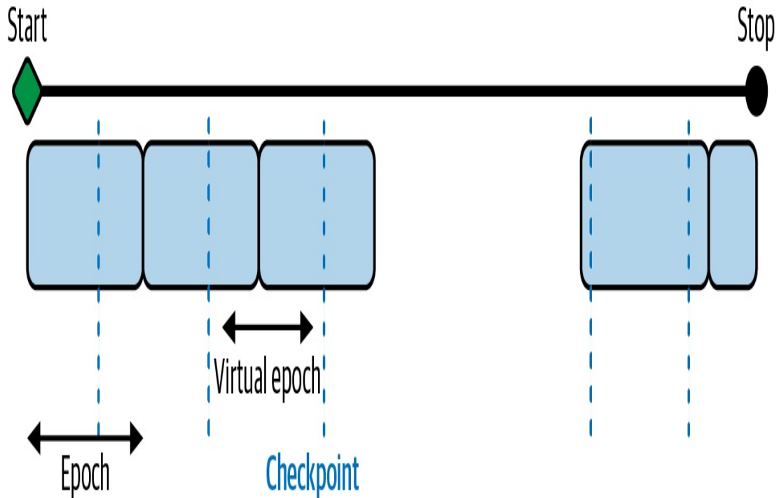
Figure 4-12. Defining a virtual epoch in terms of the desired number of steps between checkpoints.
