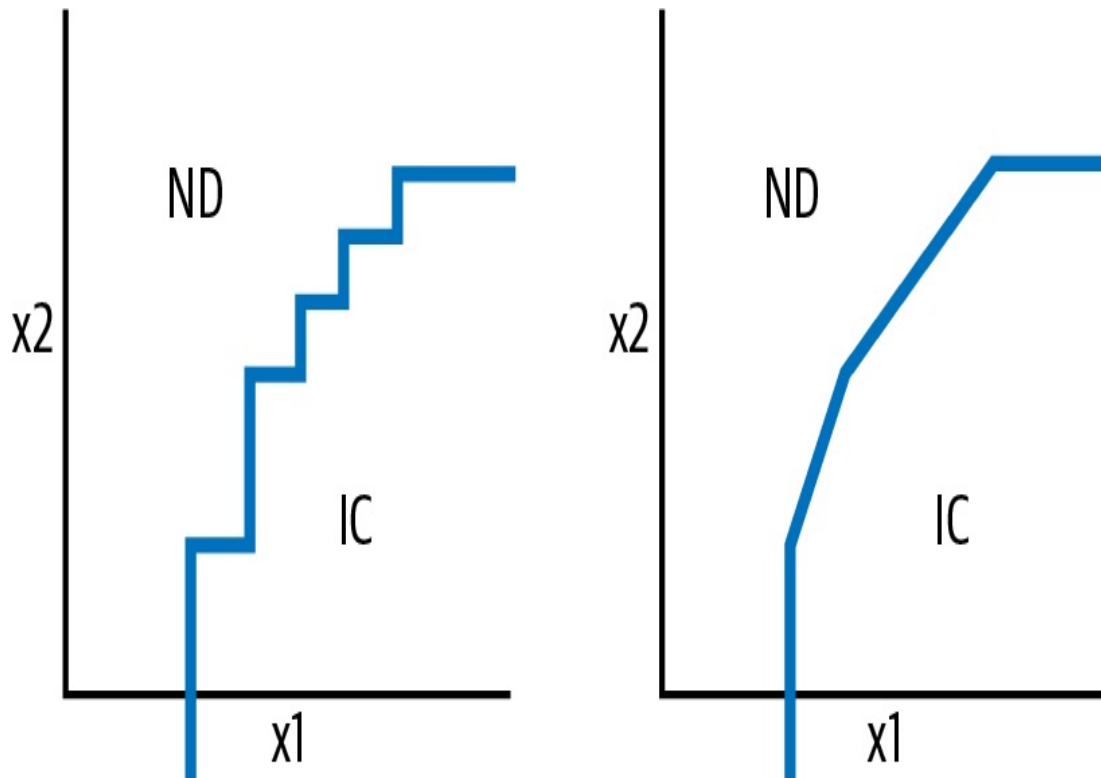
Figure 2-2. A decision tree classifier where each node can threshold only one input value ( x_1 or x_2 ) will result in a stepwise linear boundary function, whereas an oblique tree classifier where a node can threshold a linear combination of input variables will result in a piecewise linear boundary function. The piecewise linear function requires fewer nodes and can achieve greater accuracy.
