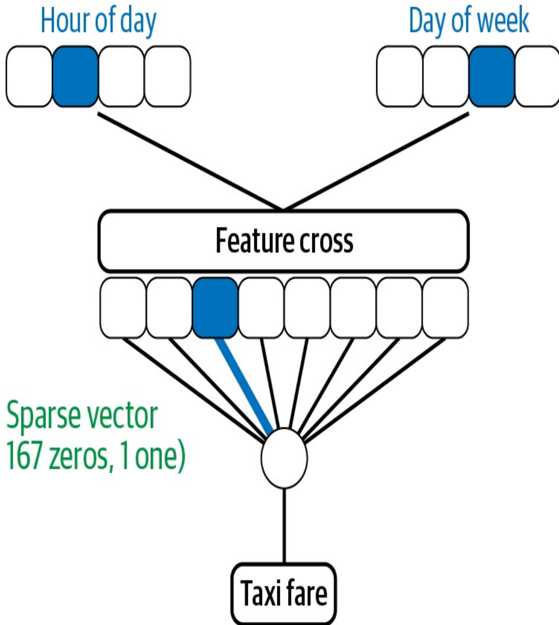
Figure 2-17. A feature cross of day_of_week and hour_of_day produces a sparse vector of dimension 168.
