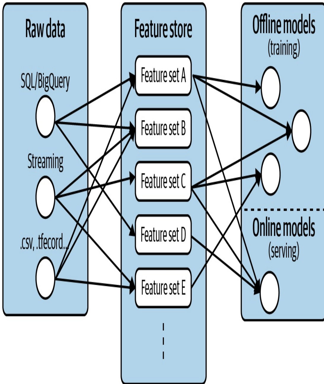
Figure 6-12. A feature store provides a bridge between raw data sources and model training and serving.
