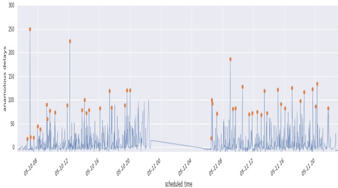
Figure 6-5. Arrival delays at Dallas Fort Worth (DFW) airport on May 10–11, 2010. Abnormal arrival delays are marked with a dot.
