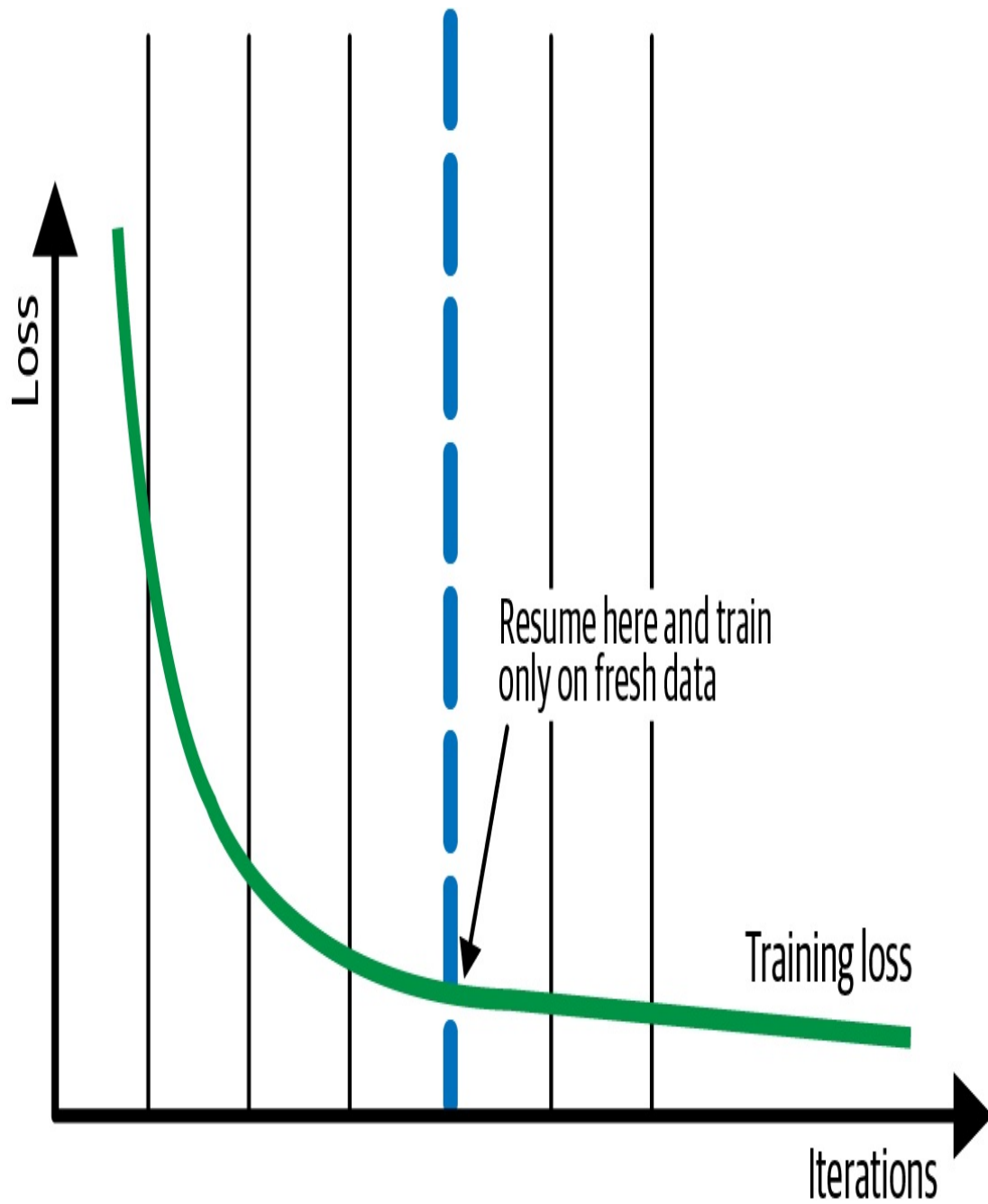
Figure 4-11. Resume from a checkpoint from before the training loss starts to plateau. Train only on fresh data for subsequent iterations.
