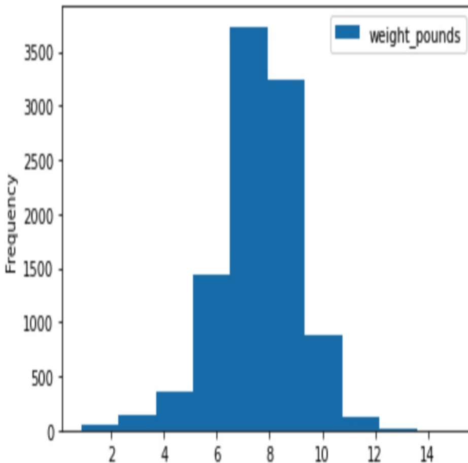
Figure 3-20. A histogram depicting the distribution of baby weight for 10,000 examples in the BigQuery natality dataset.
