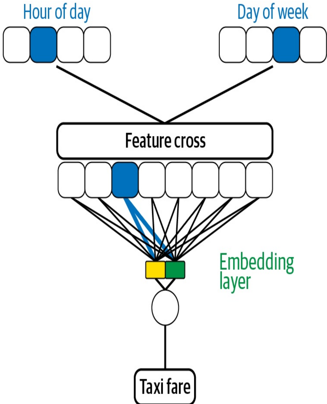
Figure 2-18. An embedding layer is a useful way to address the sparsity of a feature cross.
