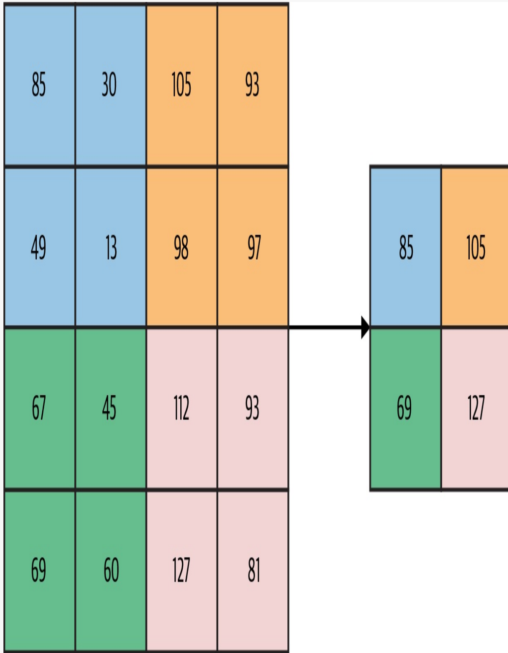
Figure 2-22. Max pooling on a single 4 \times 4 slice of image data.
