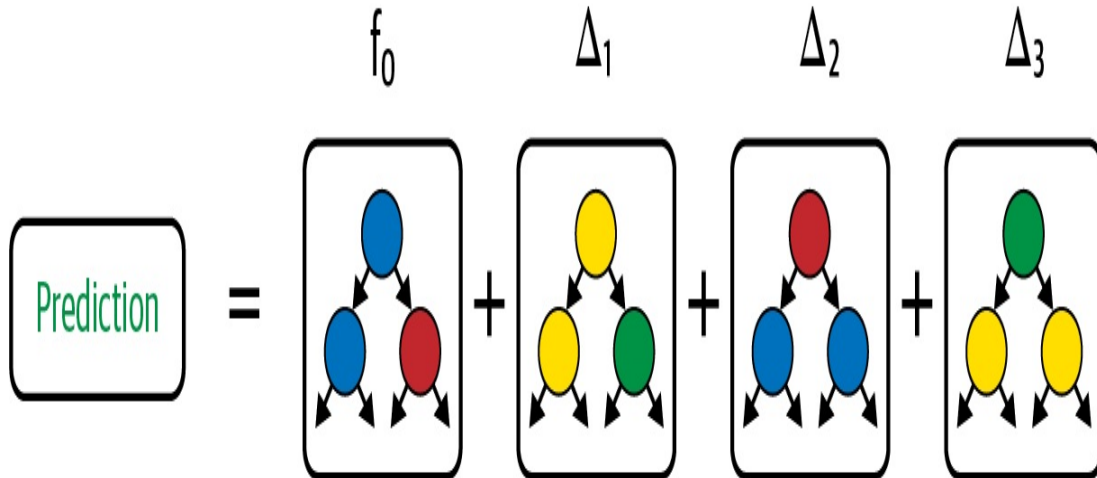
Figure 3-13. Boosting iteratively builds a strong learner from a sequence of weak learners that model the residual error of the previous iteration.
