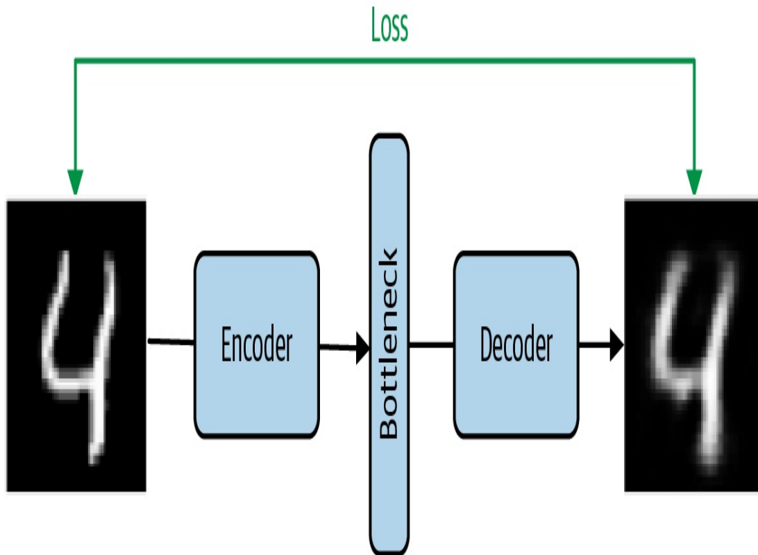
Figure 2-11. When training an autoencoder, the feature and the label are the same and the loss is the reconstruction error. This allows the autoencoder to achieve nonlinear dimension reduction.
