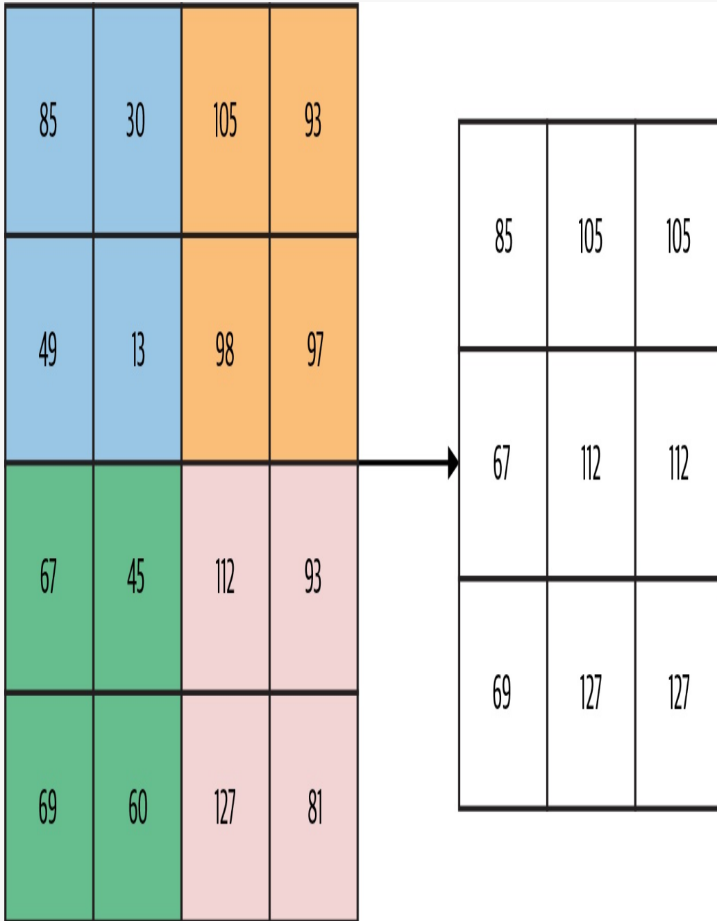
Figure 2-23. Using overlapping windows for max pooling on a 4×4 pixel grid.
