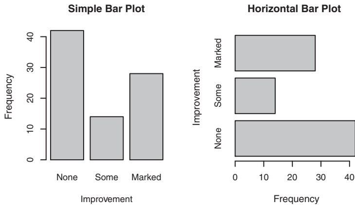
Figure 6.1 Simple vertical and horizontal bar charts
