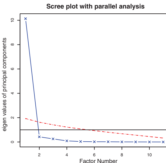
Figure 14.2 Assessing the number of principal components to retain for the USJudgeRatings example. A scree plot (the line with x's), eigenvalues greater than 1 criteria (horizontal line), and parallel analysis with 100 simulations (dashed line) suggest retaining a single component.
