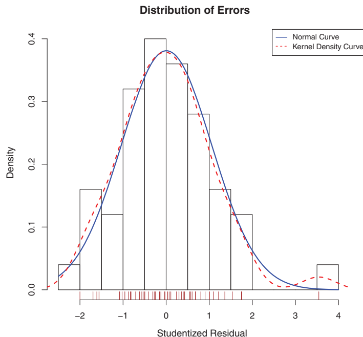
Figure 8.10 Distribution of studentized residuals using the residplot() function
