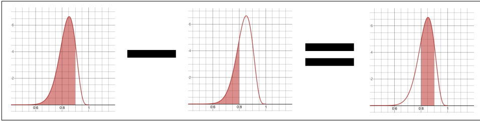
Figure 2-9. Obtaining the area between .80 and .90
