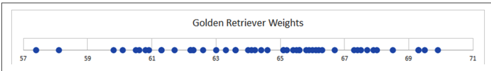
Figure 3-3. A sample of 50 golden retriever weights
