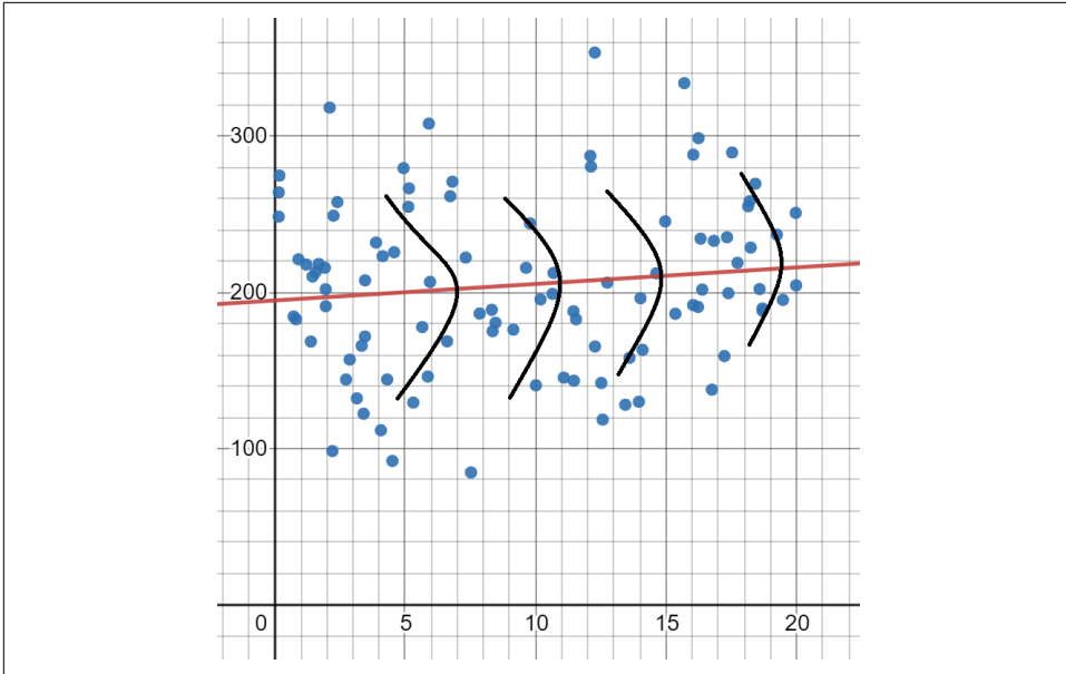
Figure 5-16. A linear regression assumes a normal distribution is following the line
