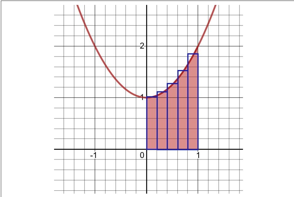
Figure 1-11. Packing rectangles under a curve to approximate area
