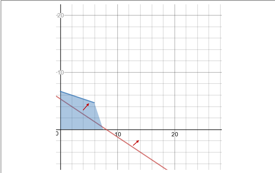
Figure A-7. Increasing our objective line until it no longer is in the feasible region
