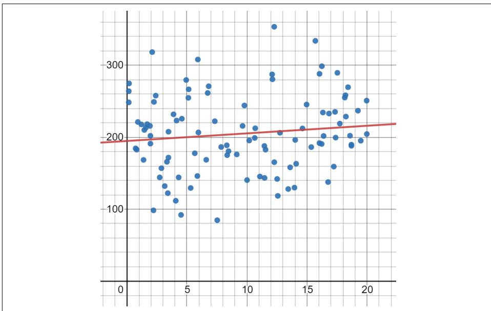
Figure 5-11. A scatterplot of data with high variance
