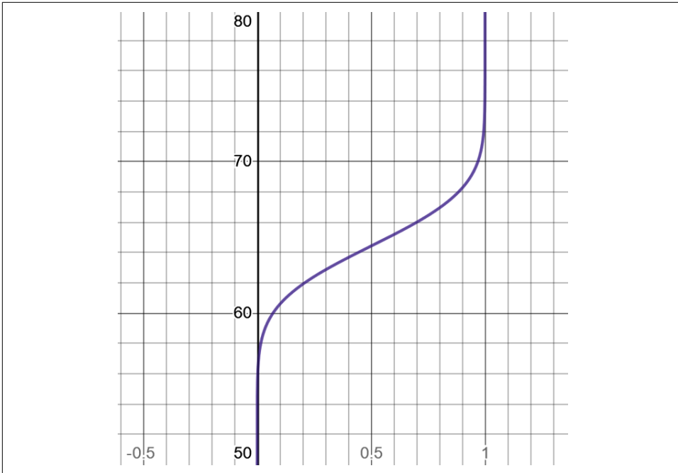
Figure 3-11. The inverse CDF, also called the PPF or quantile function
