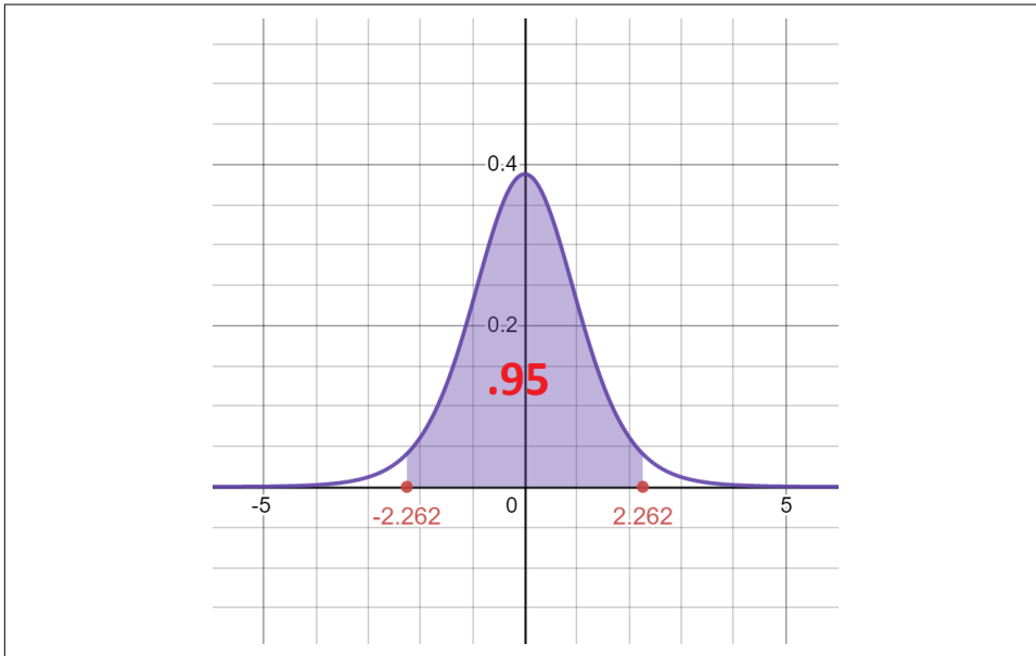
Figure 5-14. A T-distribution with 9 degrees of freedom, as there are 10 records and we subtract 1
