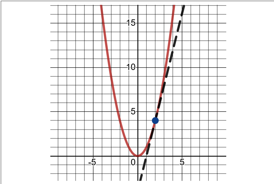
Figure 1-6. Observing steepness at a given part of the function
