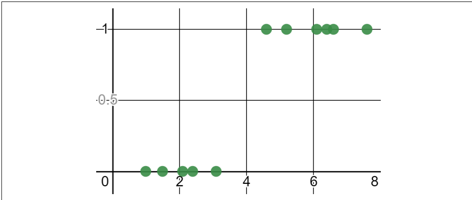
Figure 6-1. Plotting whether patients showed symptoms (1) or not (0) over x hours of exposure
