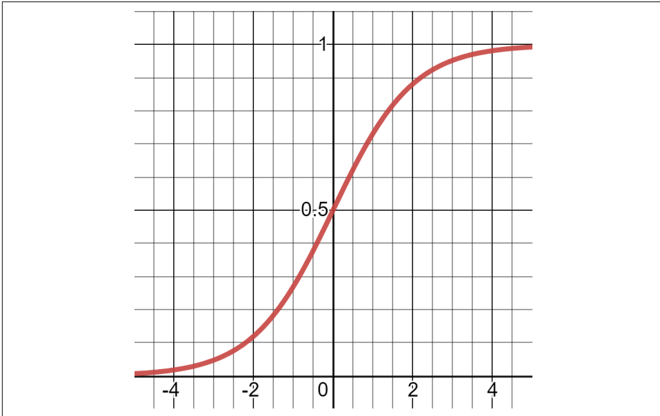
Figure 7-7. Logistic activation function
