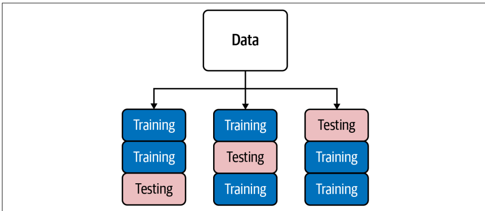
Figure 6-15. A three-fold cross-validation alternating each third of the dataset as a testing dataset
