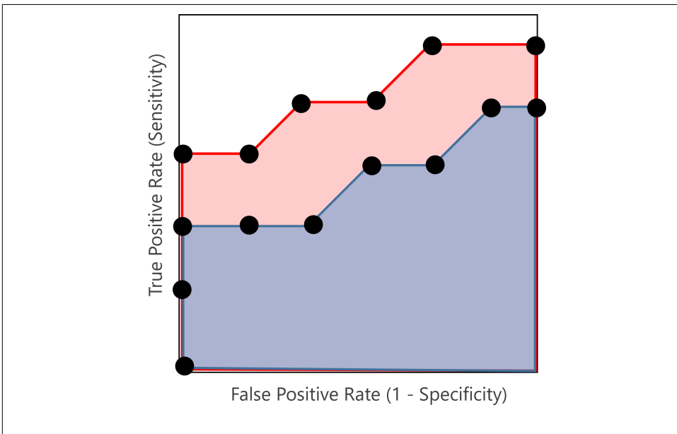
Figure 6-21. Comparing two models by their area under the curve (AUC) with their respective ROC curves
