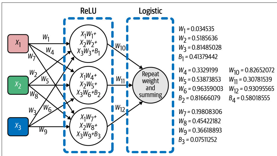
Figure 7-9. Visualizing our neural network against the weight and bias matrix values
