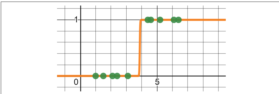
Figure 6-13. This logistic regression has a perfect R^2 of 1.0 because there is a clean divide in outcomes predicted by hours of exposure
