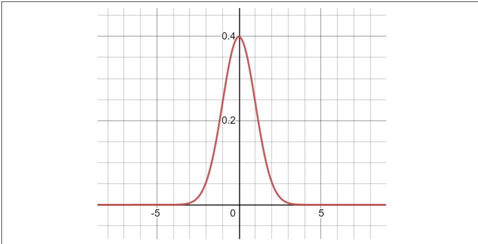
Figure A-4. Most values in a standard normal distribution are small and near 0, while larger values are less frequent on the tails
