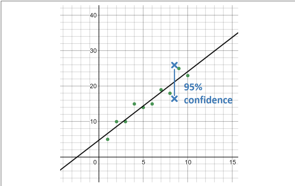
Figure 5-17. A prediction interval for a dog that is 8.5 years old with 95% confidence
