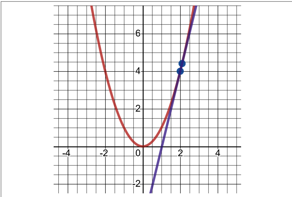
Figure 1-7. A crude way of calculating slope
