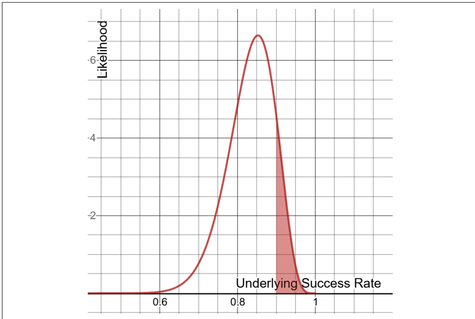
Figure 2-7. Beta distribution after 30 successes and 6 failures
