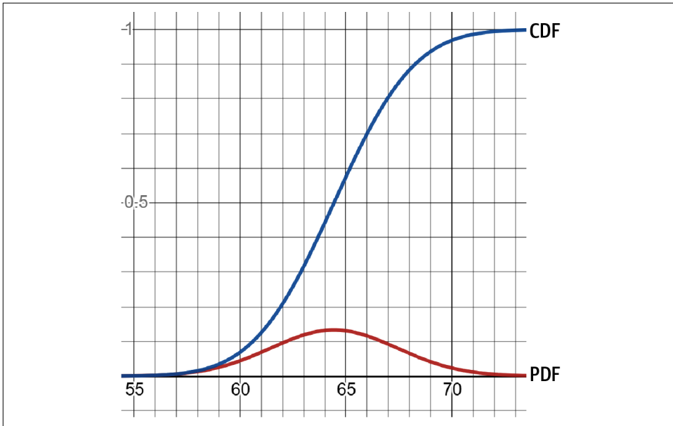
Figure 3-8. A PDF alongside its CDF
