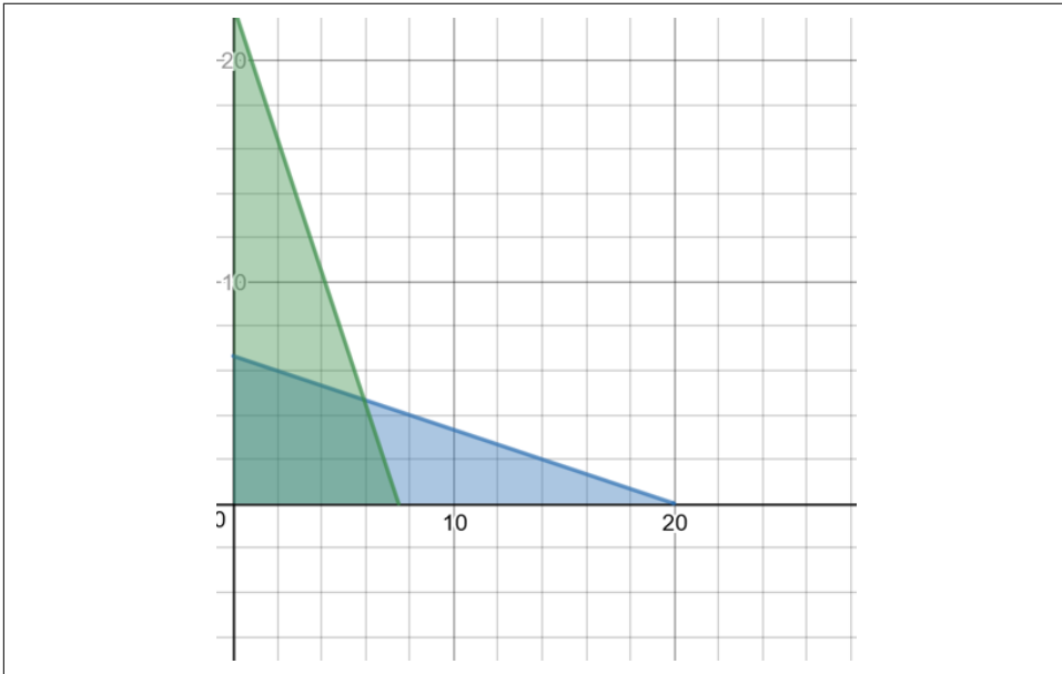
Figure A-6. Graphing the second constraint
