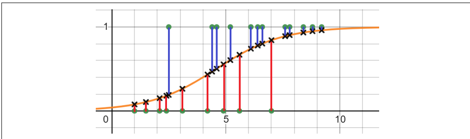
Figure 6-11. Projecting the output values back onto the logistic curve
