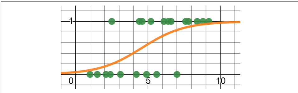
Figure 6-12. Our data has a mediocre R^2 of 0.30645 because there is a lot of variance in the middle of our curve
