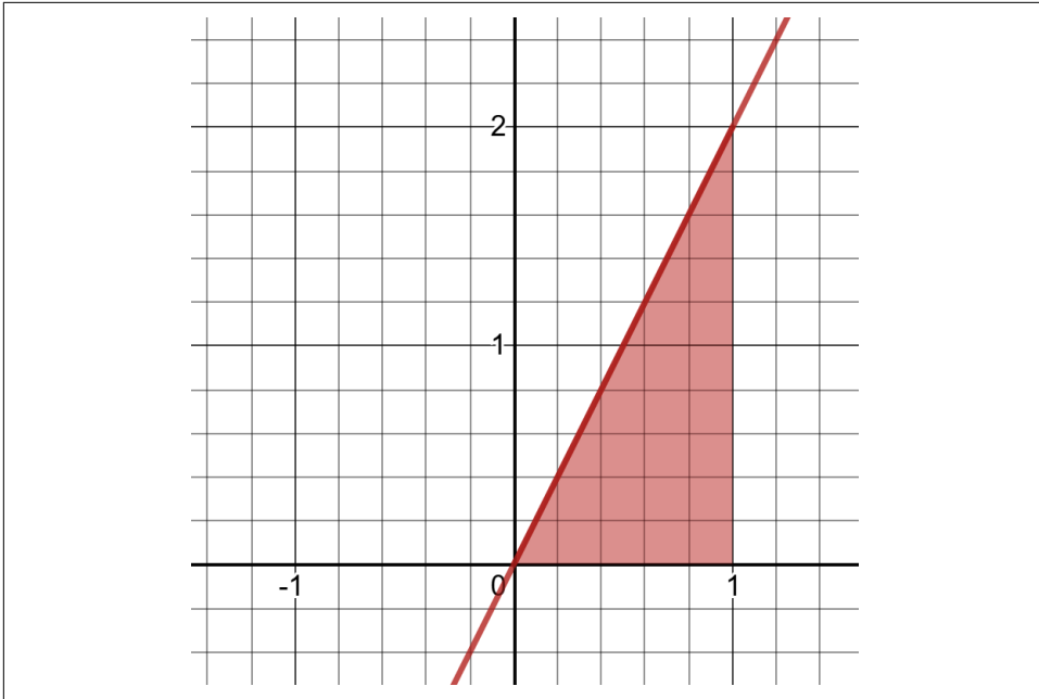
Figure 1-9. Calculating an area under a linear function
