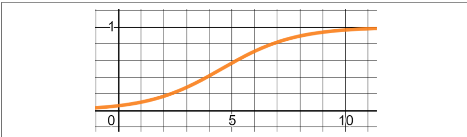
Figure 6-6. A logistic function
