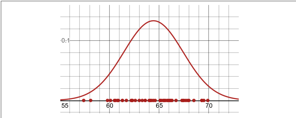
Figure 3-6. A normal distribution fitted to data points
