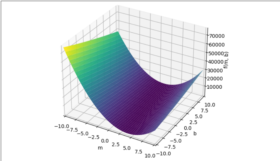
Figure 5-9. The loss landscape for a simple linear regression
