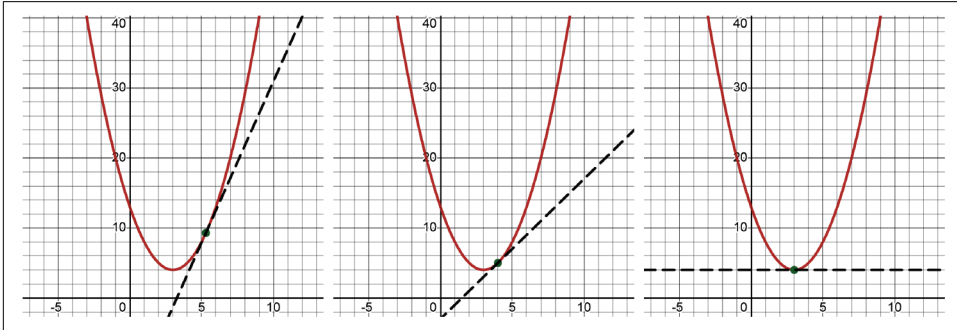
Figure 5-8. Stepping toward the local minimum where the slope approaches 0
