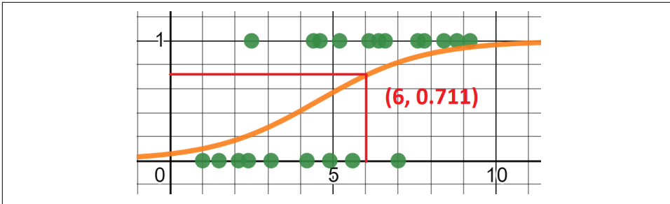
Figure 6-5. We can expect a patient exposed for six hours to be 71.1% likely to have symptoms, and because that's greater than a threshold of 50% we predict they will show symptoms
