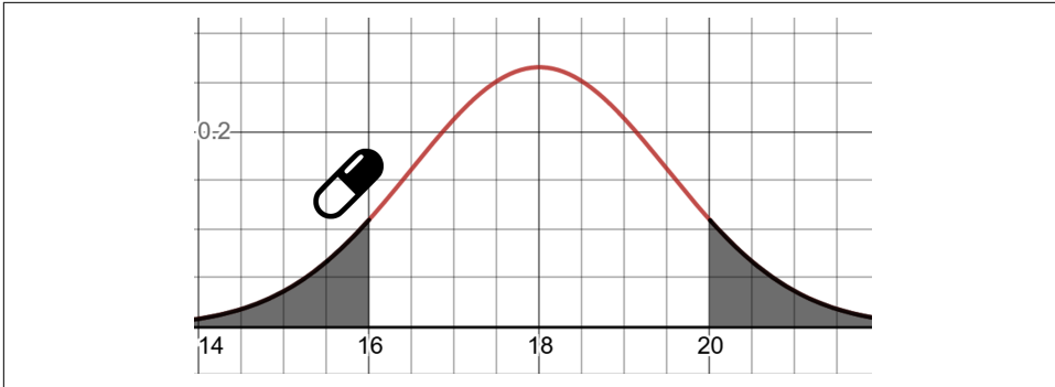
Figure 3-23. The p-value adds symmetrical sides for statistical significance
