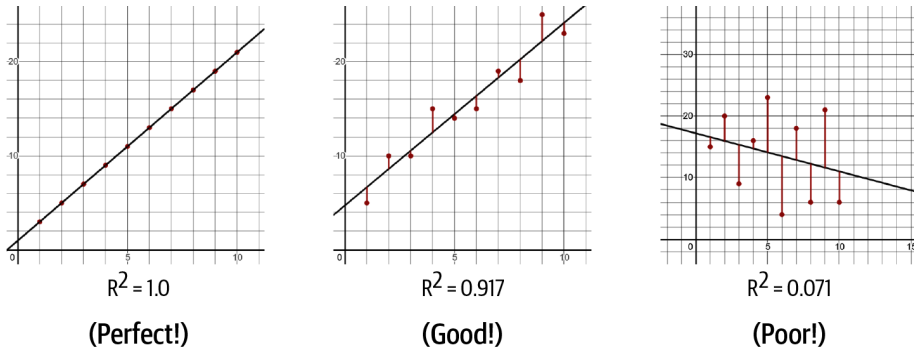
Figure 5-19. An r^2 applied to different testing datasets with a trained linear regression
