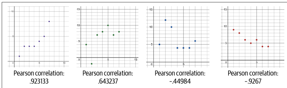
Figure 5-12. Correlation coefficients for four scatterplots
