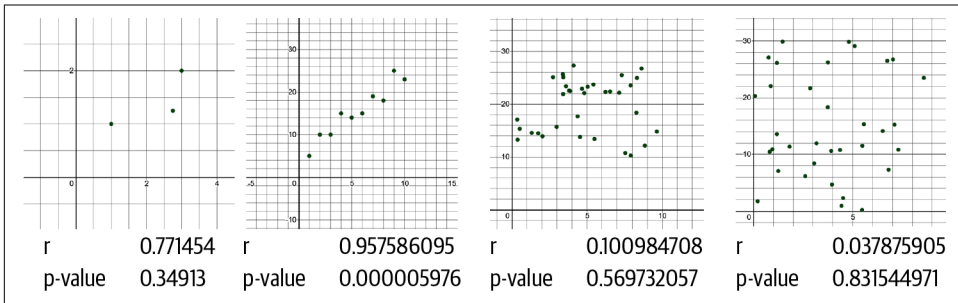
Figure 5-15. Different datasets and their correlation coefficients and p-values
