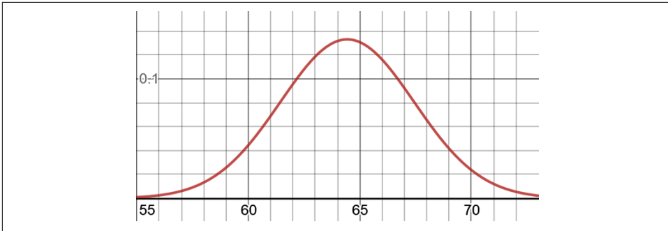
Figure 3-2. A normal distribution
