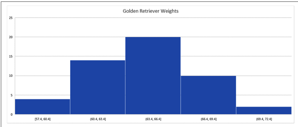
Figure 3-5. A more productive histogram
