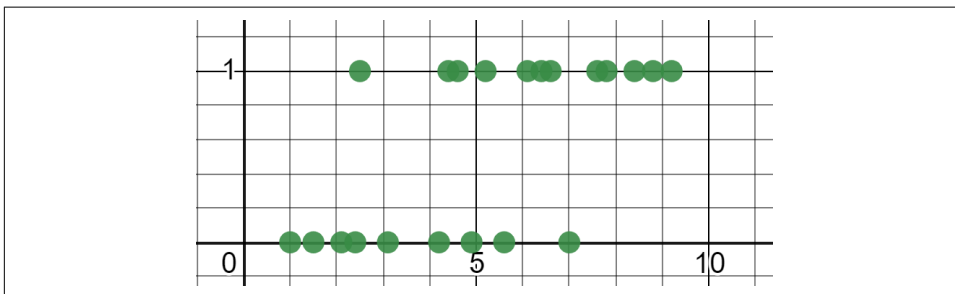
Figure 6-3. A mix of patients who show symptoms (1) and do not show symptoms (0) exists in the middle
