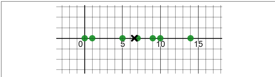
Figure 3-1. Visualizing the spread of our data, where "X" is the mean
