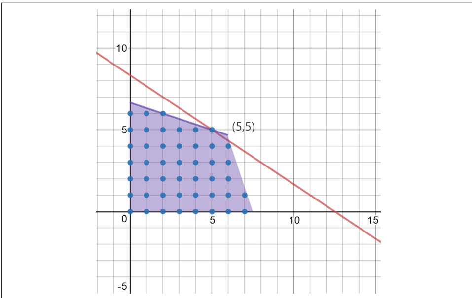
Figure A-9. A discrete linear programming system
