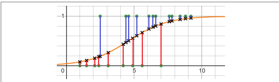
Figure 6-8. Every input value has a corresponding likelihood on the logistic curve
