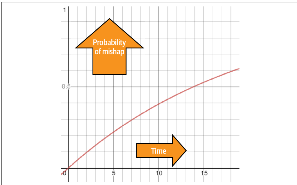
Figure A-3. Predicting the probability of a leak over time
