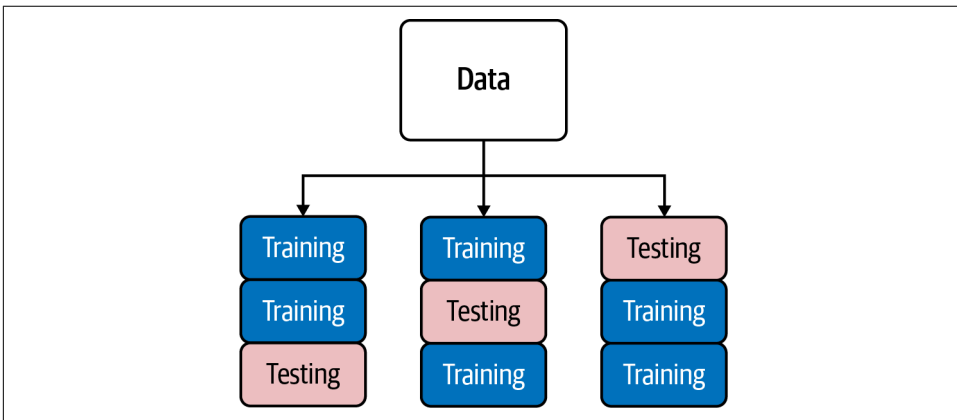
Figure 5-20. A visualization of cross-validation with three folds
