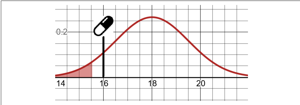
Figure 3-19. We have failed to prove our drug test result is statistically significant
