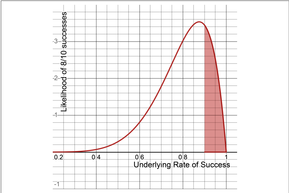
Figure 2-5. The probability of success being 90% or more
