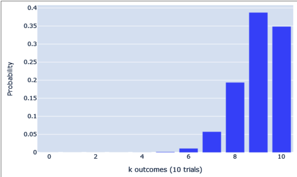
Figure 2-1. A binomial distribution
