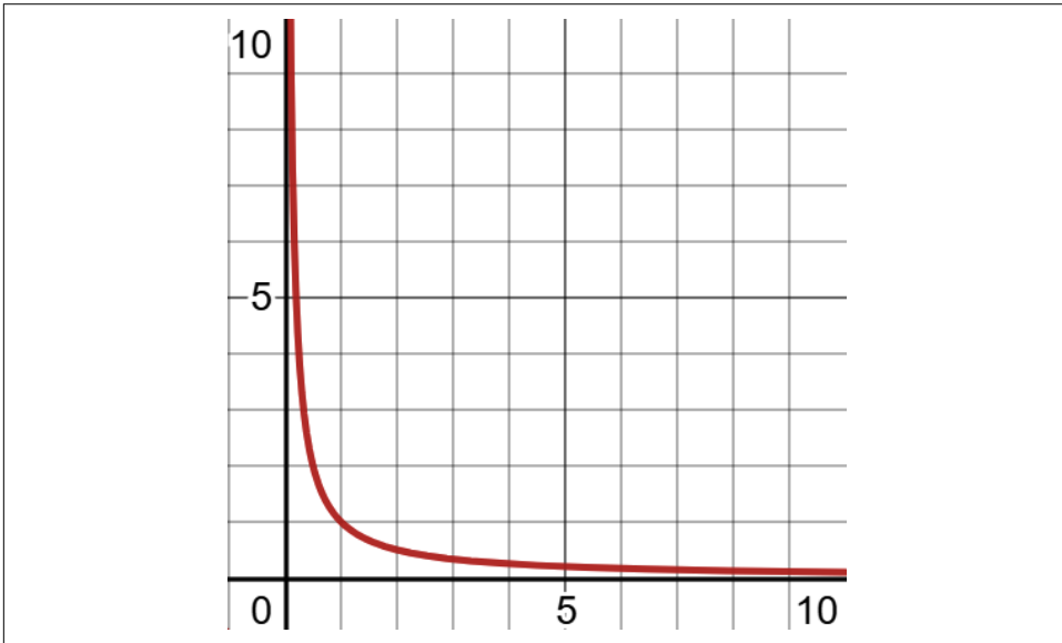
Figure 1-5. A function that forever approaches 0 but never reaches 0
