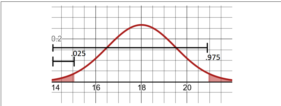
Figure 3-21. Calculating the central 95% of normal distribution area
