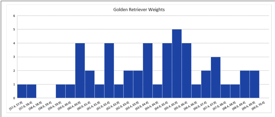
Figure 3-4. A histogram of golden retriever weights
