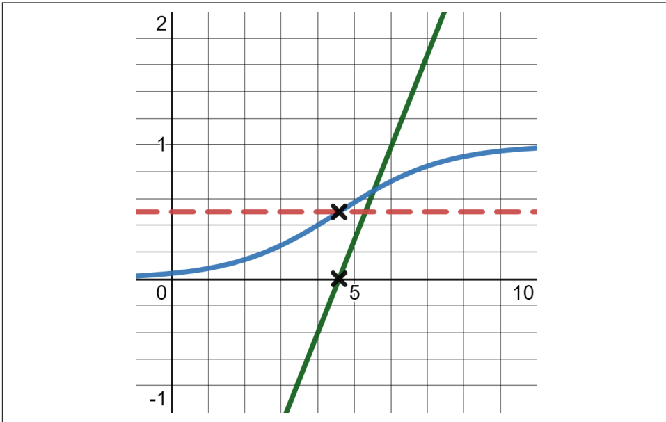
Figure 6-10. The log-odds line is converted into a logistic function that outputs a probability
