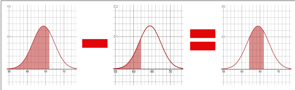
Figure 3-10. Finding a middle range of probability
