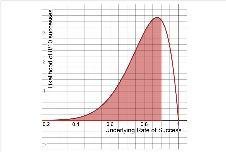
Figure 2-4. Calculating the area up to 90% (0.0 to 0.90)
