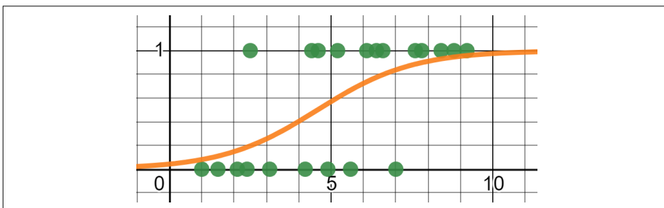
Figure 6-4. Fitting a logistic function to the data
