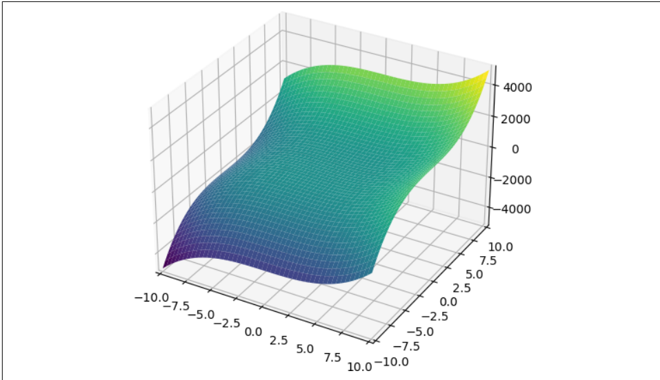
Figure 1-8. Plotting a three-dimensional exponential function
