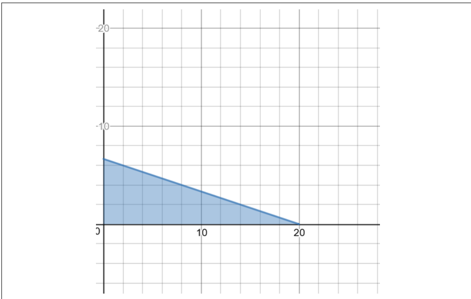
Figure A-5. Graphing the first constraint
