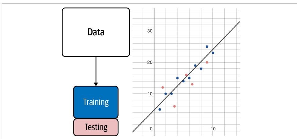
Figure 5-18. Splitting into training/testing data—the line is fitted to the training data (dark blue) using least squares, while the testing data (light red) is analyzed afterward to see how off the predictions are on data that was not seen before
