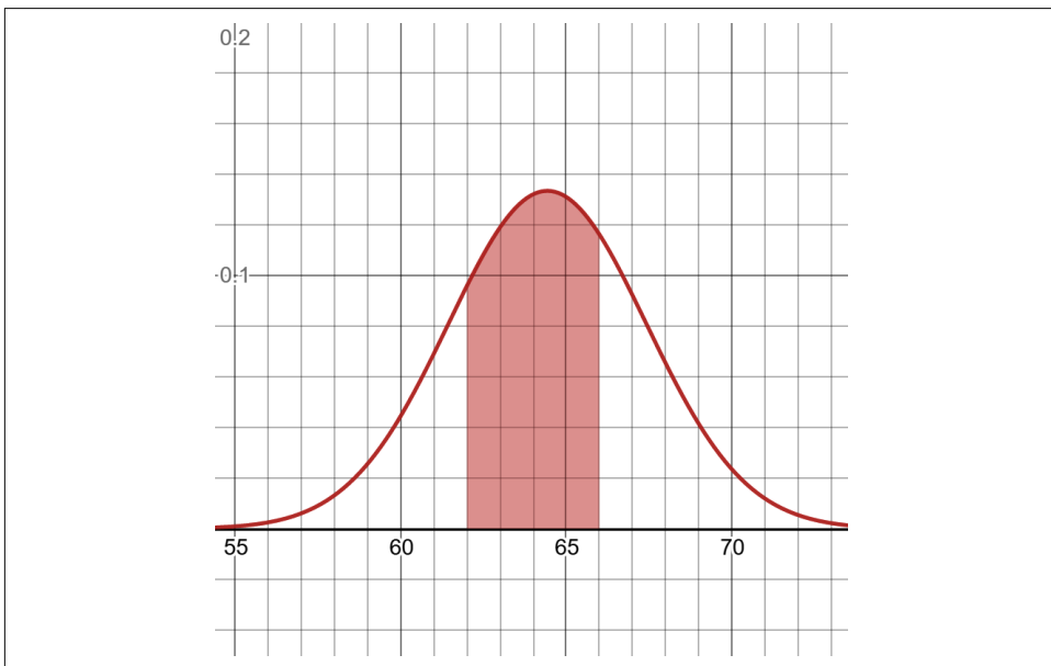
Figure 3-7. A CDF measuring probability between 62 and 66 pounds
