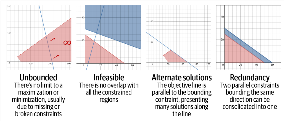
Figure A-10. Special cases of linear programming
