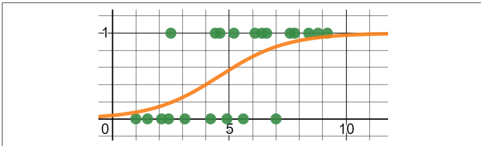
Figure 6-7. Plotting the logistic regression
