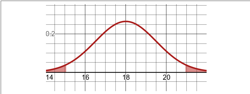
Figure 3-20. A two-tailed test
