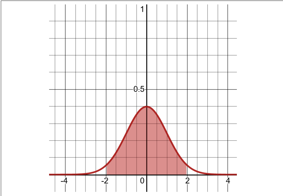
Figure 3-14. 95% symmetrical probability in the center of a standard normal distribution
