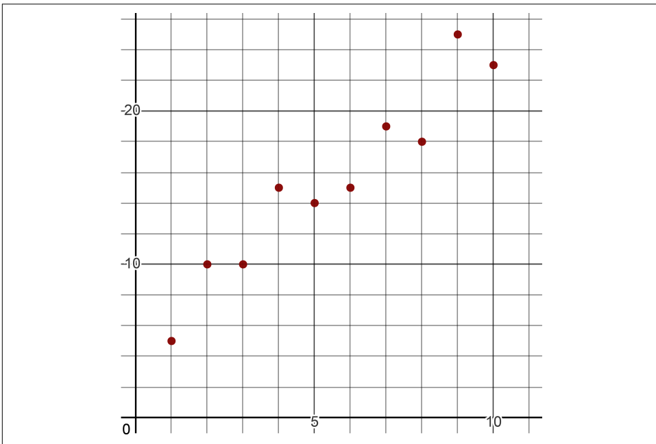
Figure 5-13. How likely would we see this data, which seems to have a linear correlation, by random chance?
