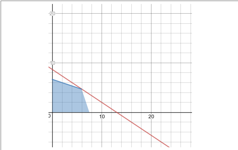
Figure A-8. Maximized objective for our linear programming system
