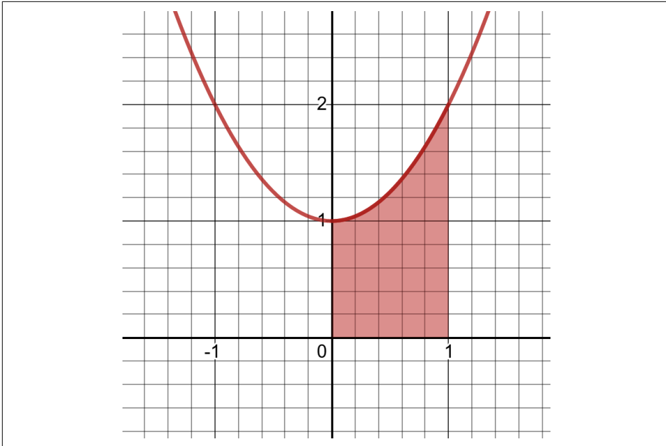
Figure 1-10. Calculating area under nonlinear functions is less straightforward
