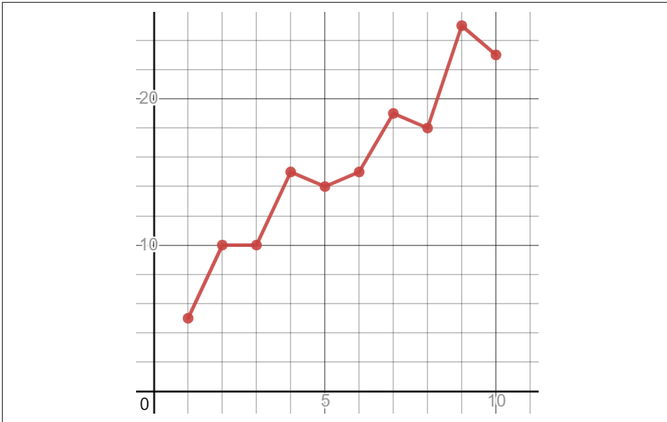
Figure 5-10. Performing a regression by simply connecting the points, resulting in zero loss
